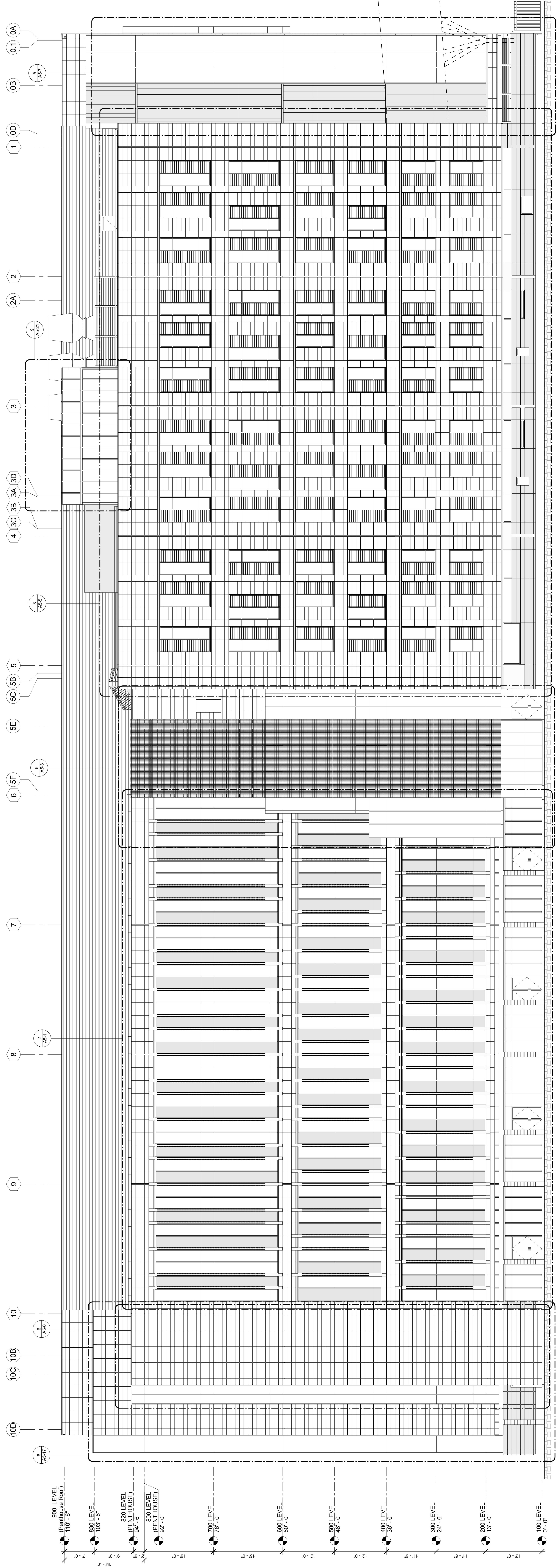
1 WEST ELEVATION A4-0 1/8" = 1'-0"
