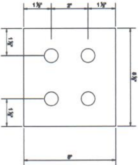
CLIP DETAIL
