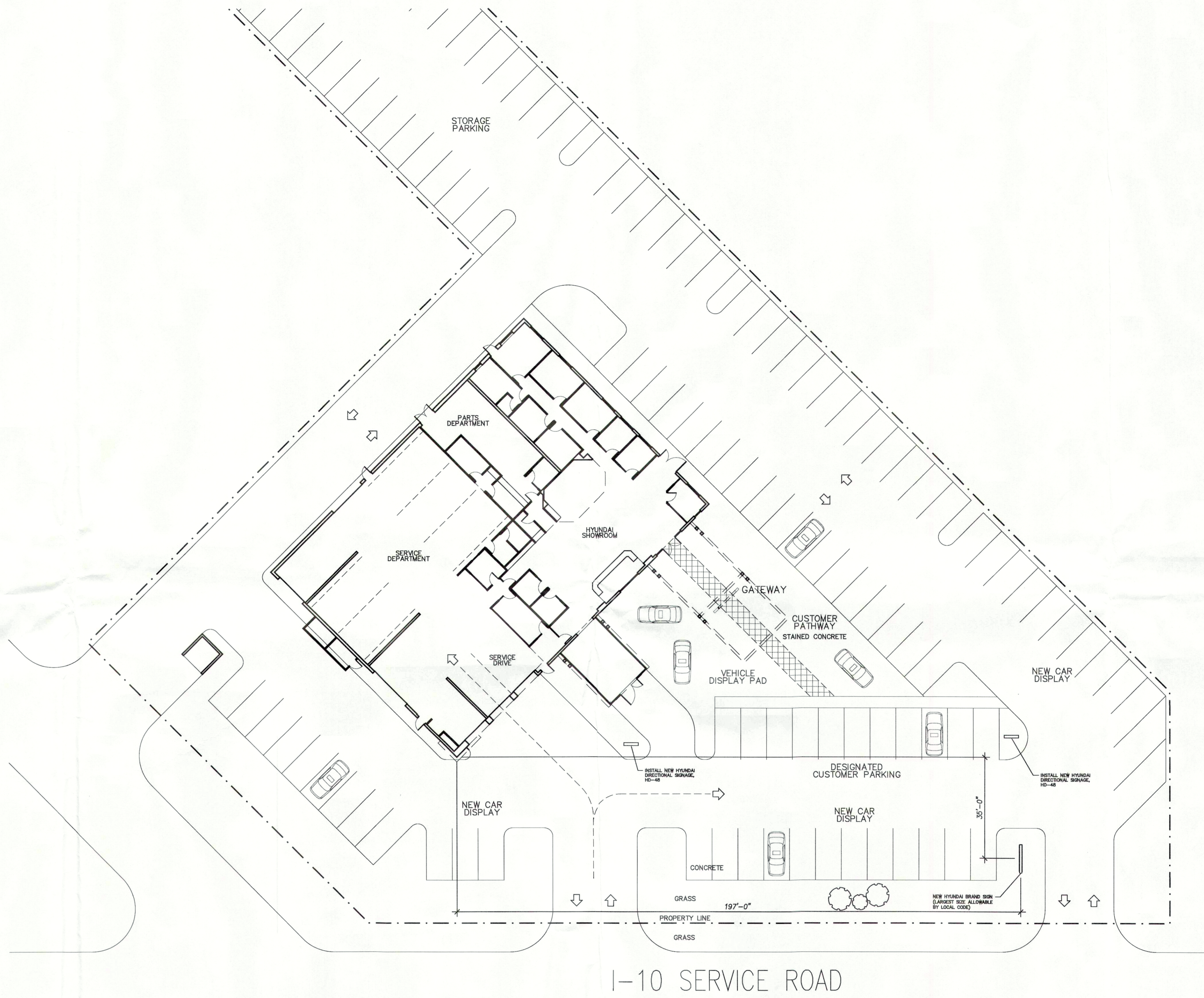
NORTH PROPOSED SITE DIAGRAM SCALE: 1" = 20'-0"
