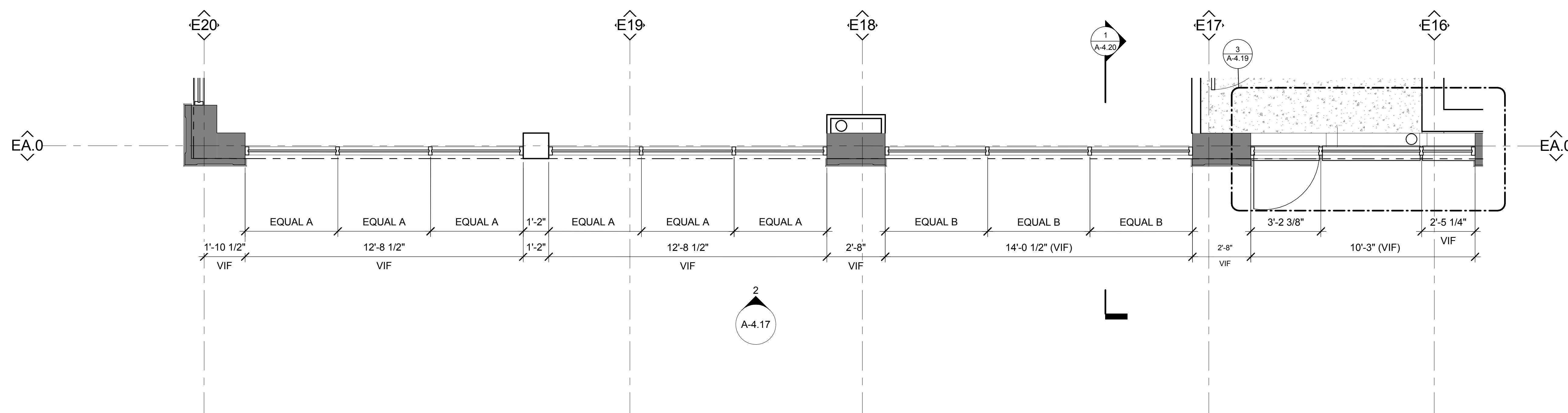
1101 ENLARGED PLAN AT RAMPART STREET - SOUTH SIDE
