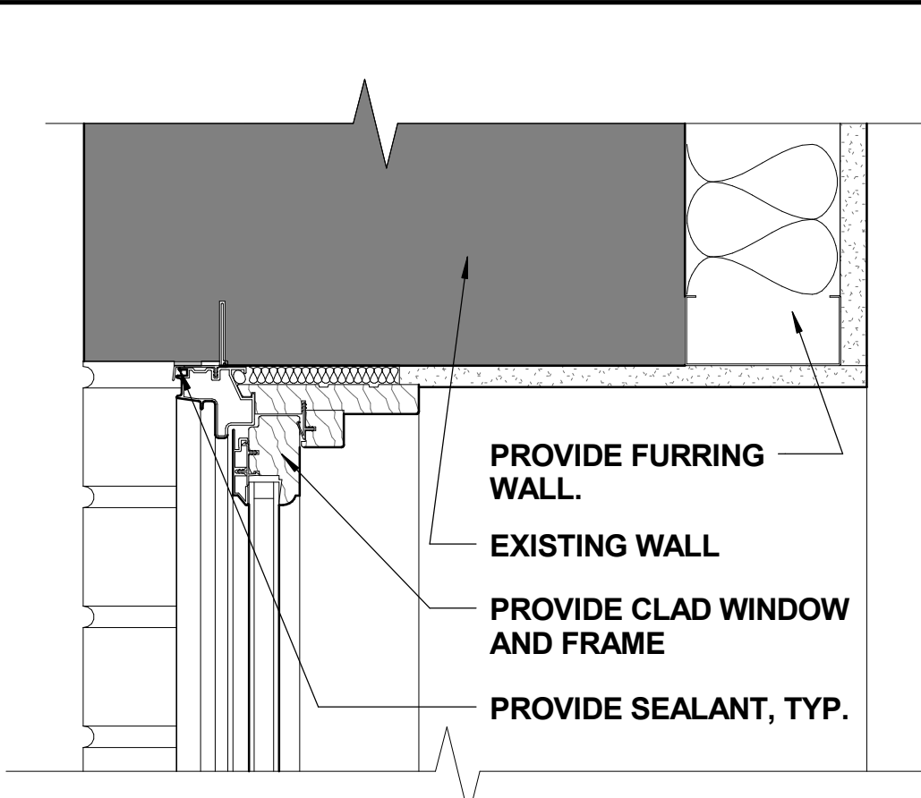
TYPE A - HEAD DETAIL 3" = 1'-0" 19
