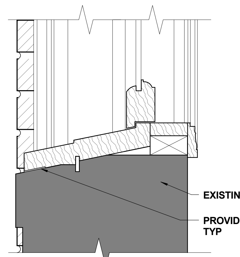
TYPE N - SILL DETAIL 3" = 1'-0" 5
