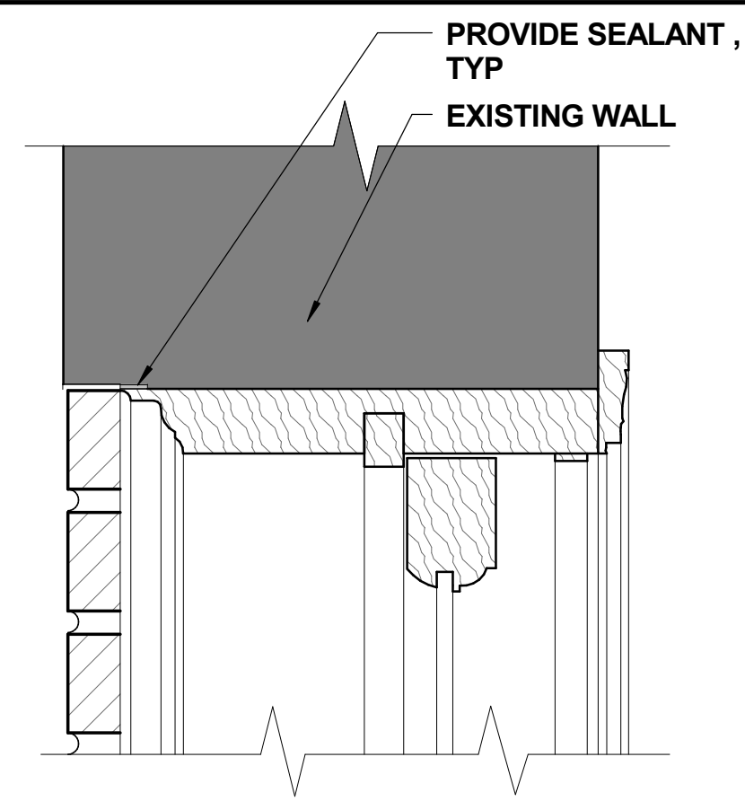
TYPE N - HEAD DETAIL 3" = 1'-0" 7
