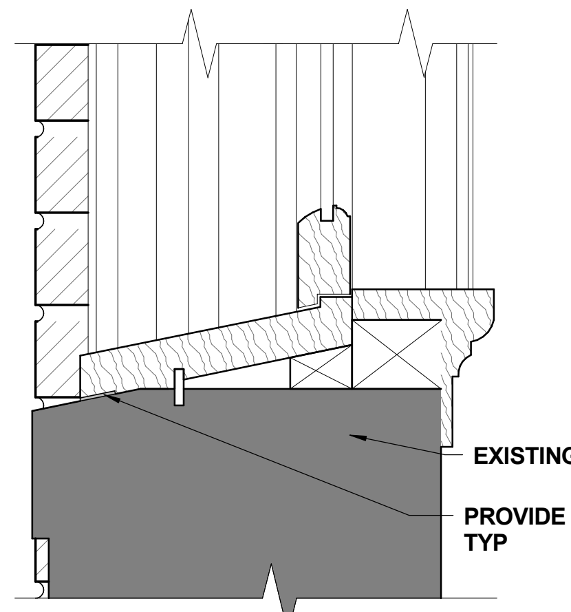
WINDOW G1 - SILL DETAIL 3" = 1'-0" 9
