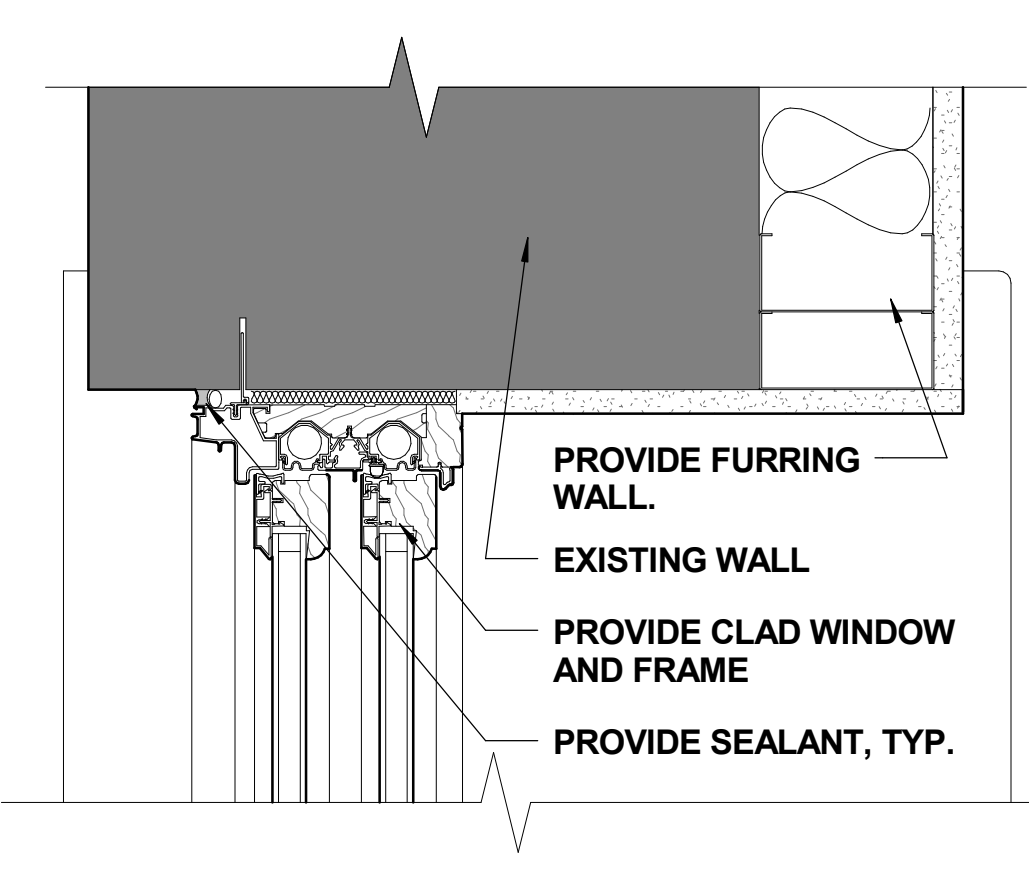
TYPE A - JAMB DETAIL 3" = 1'-0" 18
