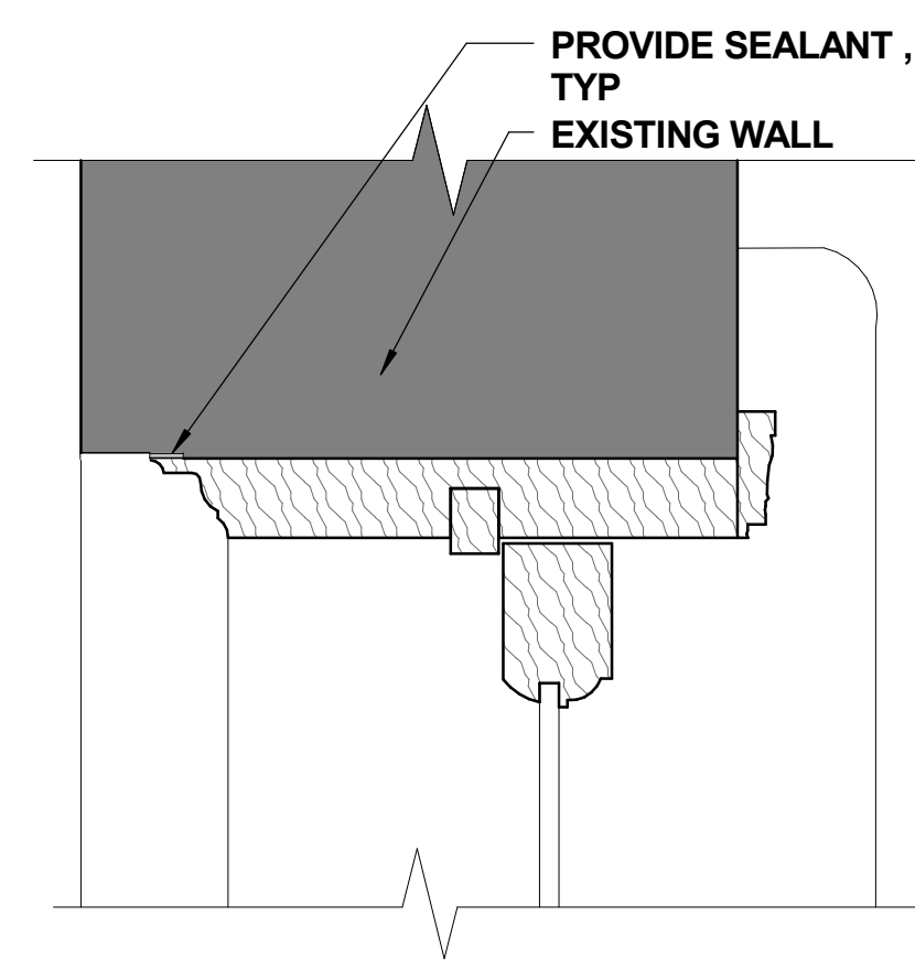
TYPE N - JAMB DETAIL 3" = 1'-0" 6
