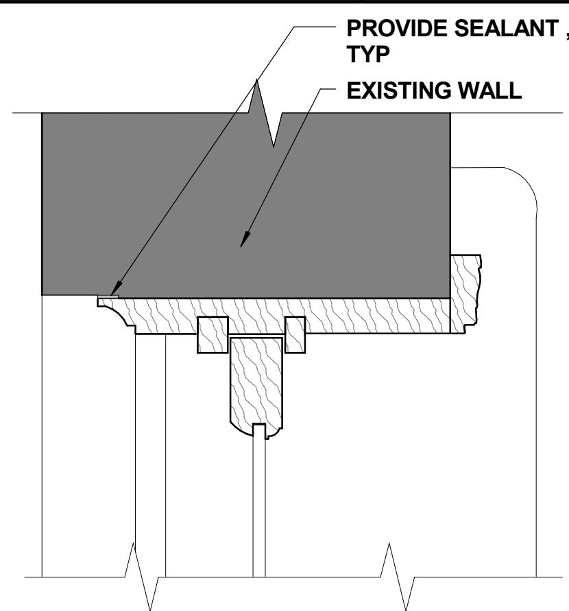
TYPE G - HEAD DETAIL 3" = 1'-0" 12
