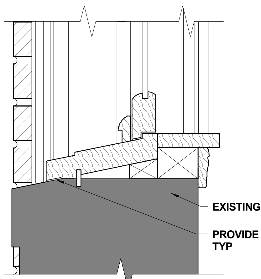
TYPE E - SILL DETAIL 3" = 1'-0" 13
