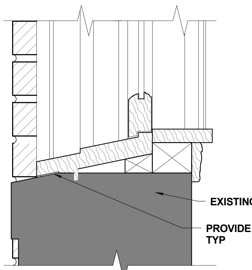
TYPE F - SILL DETAIL 3" = 1'-0" 1
