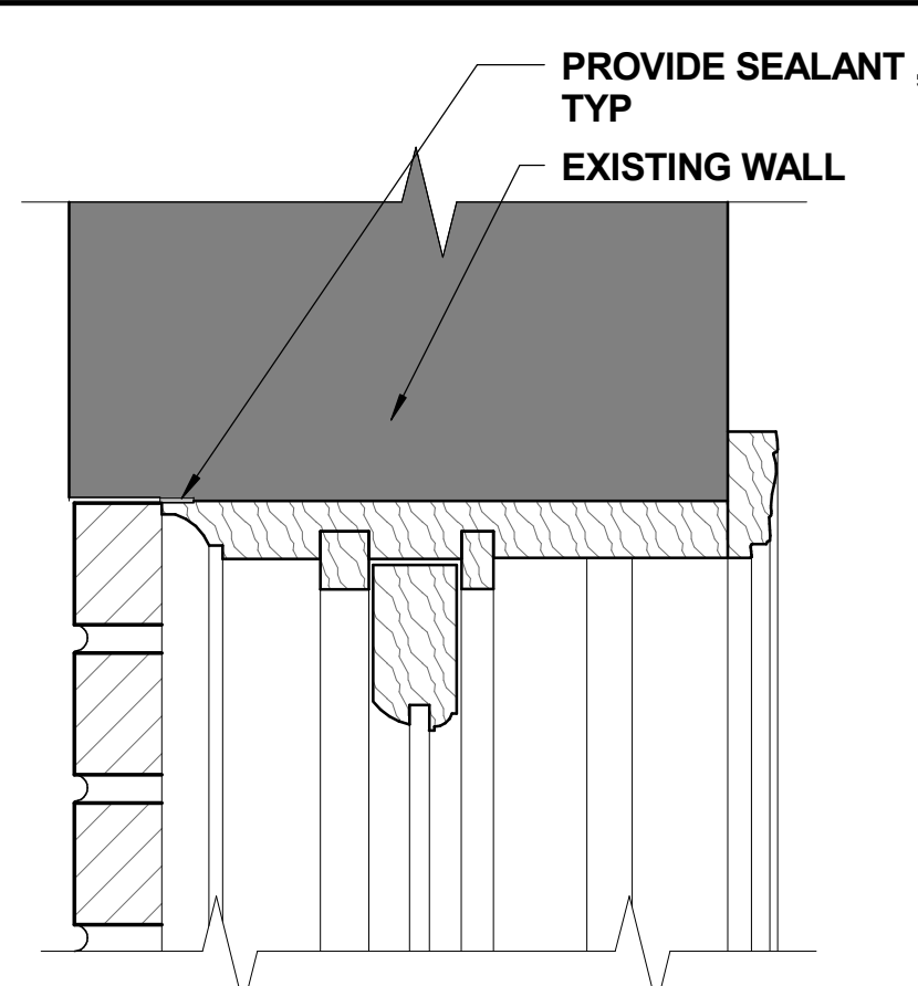
TYPE F - HEAD DETAIL 3" = 1'-0" 3
