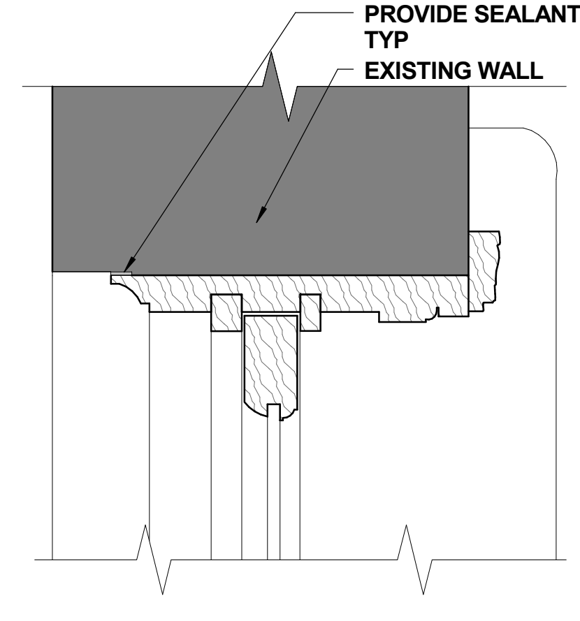
TYPE F - JAMB DETAIL 3" = 1'-0" 2
