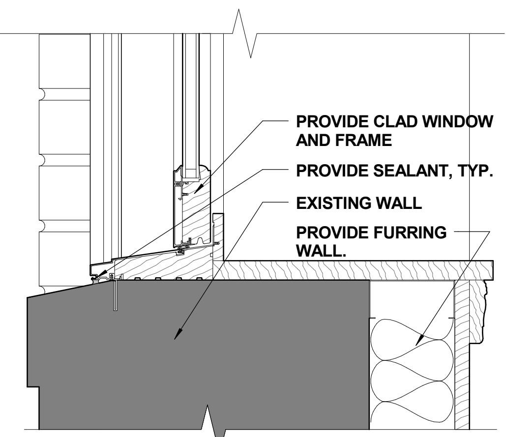
TYPE A - SILL DETAIL 3" = 1'-0" 17
