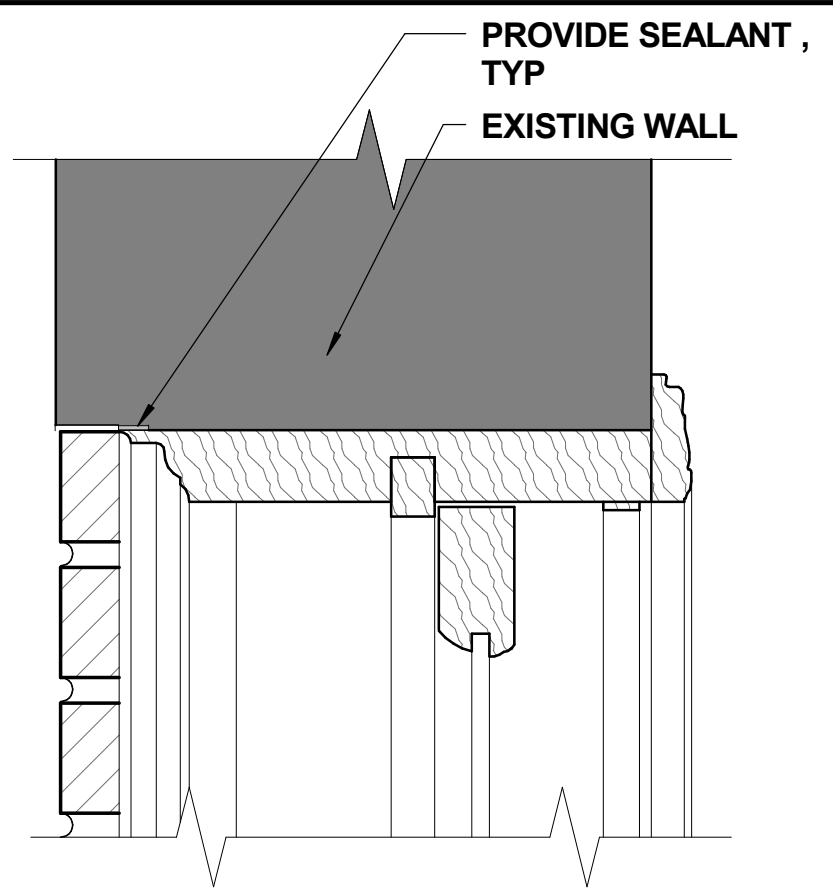
TYPE E - HEAD DETAIL 3" = 1'-0" 15
