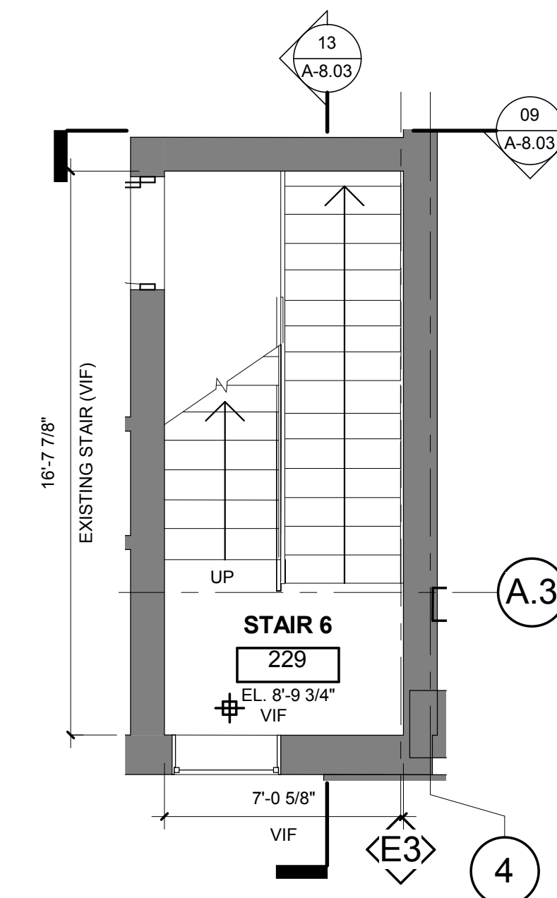
STAIR-6 2nd floor
