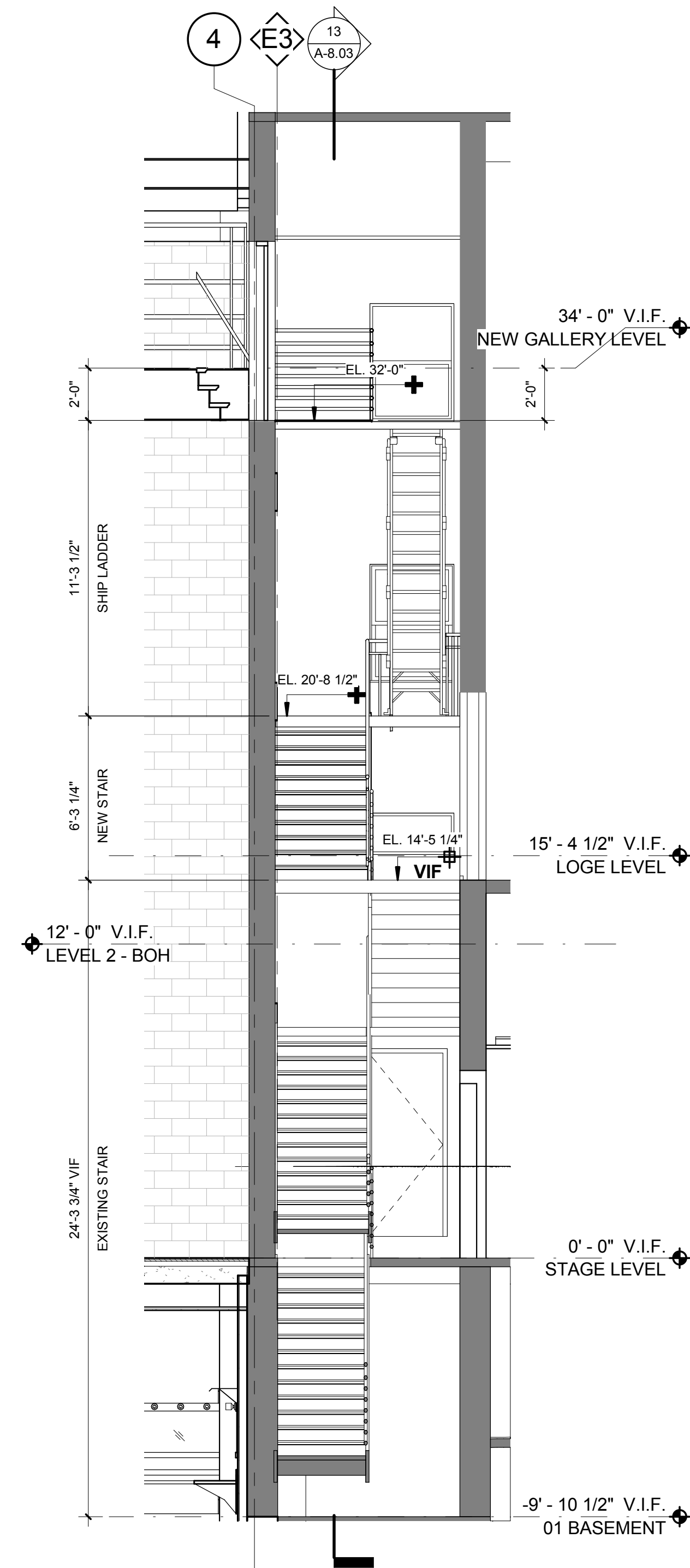
STAIR 6 - B SECTION
