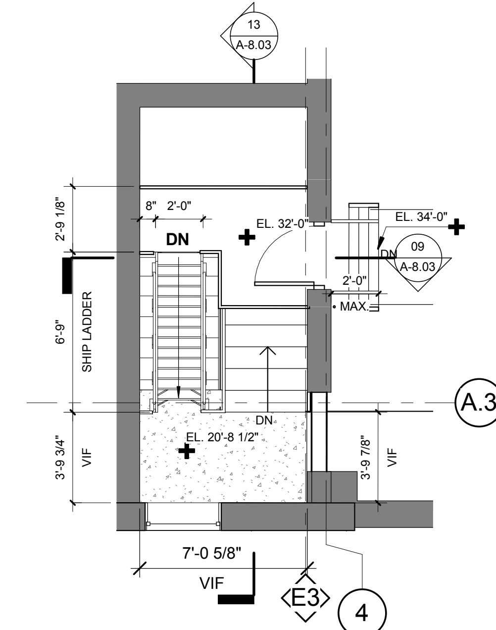
STAIR-6 - MID BALCONY
