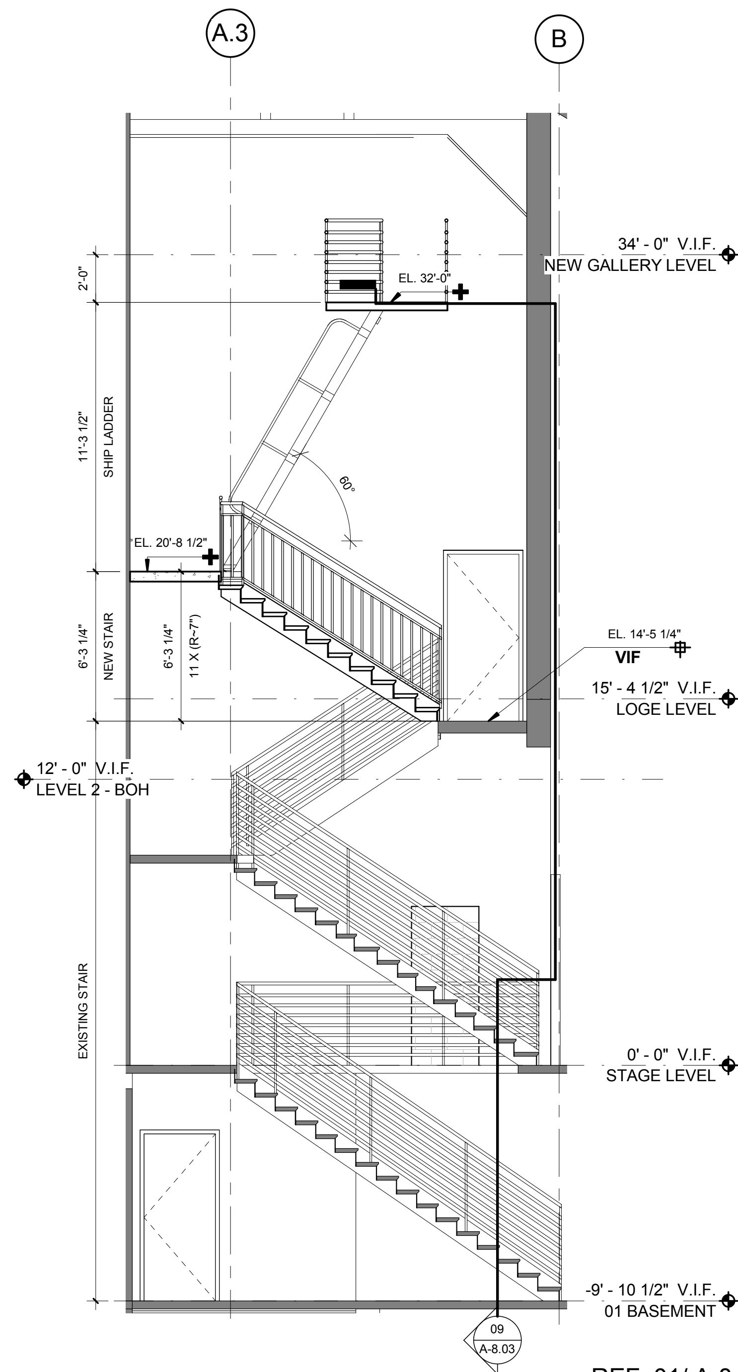
STAIR 6 - A SECTION
