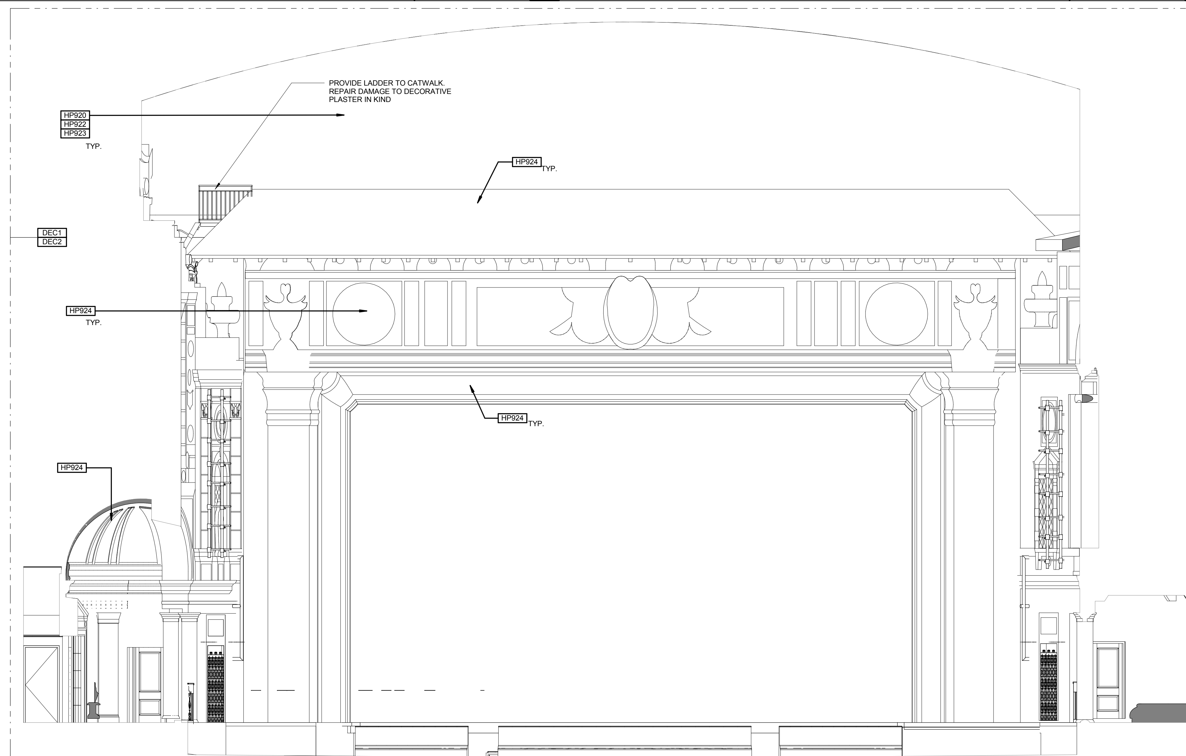
INTERIOR ELEVATION - PROSCENIUM 3/16" = 1'-0" 01
