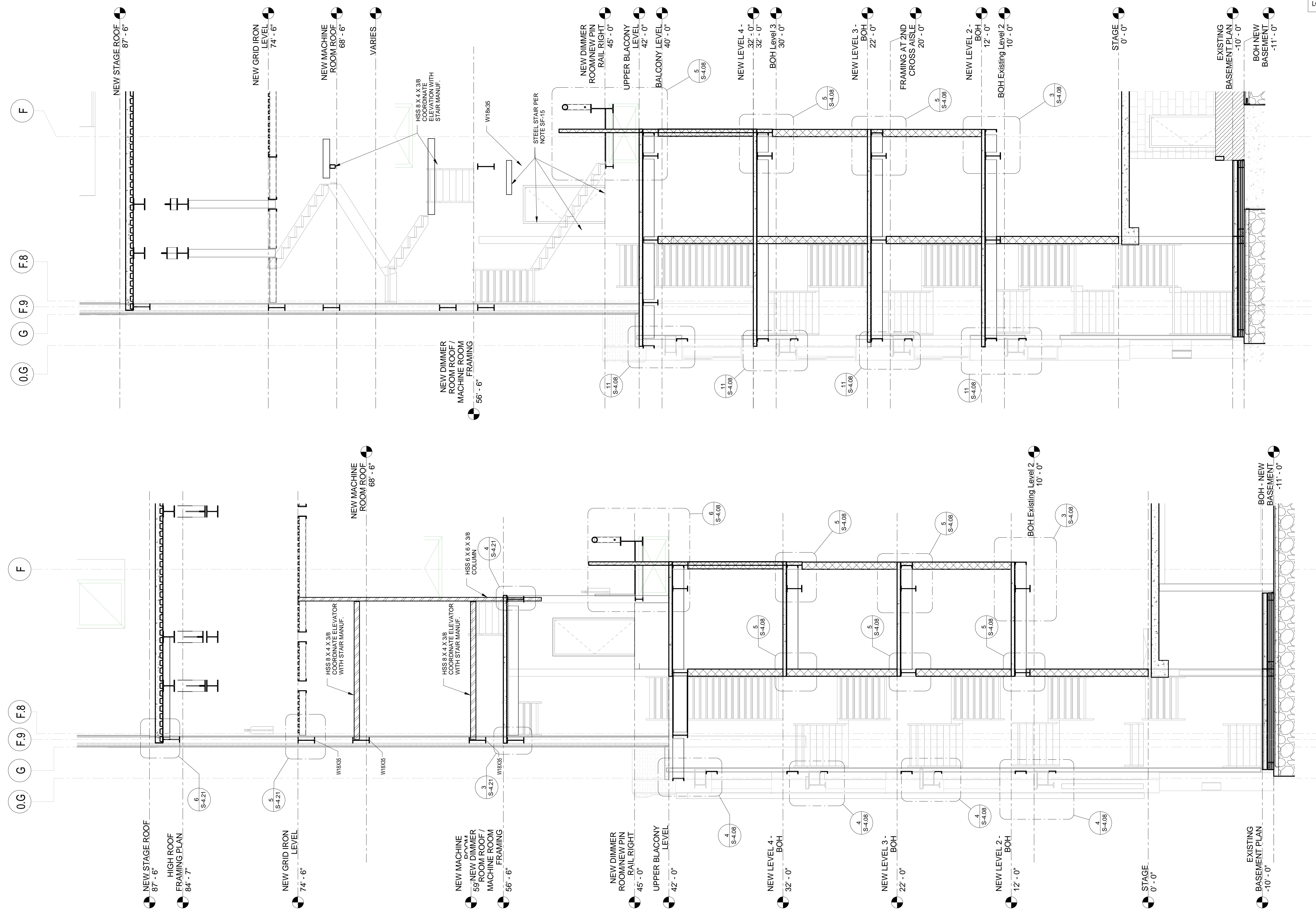
2 SECTION 1/4" = 1'-0"
