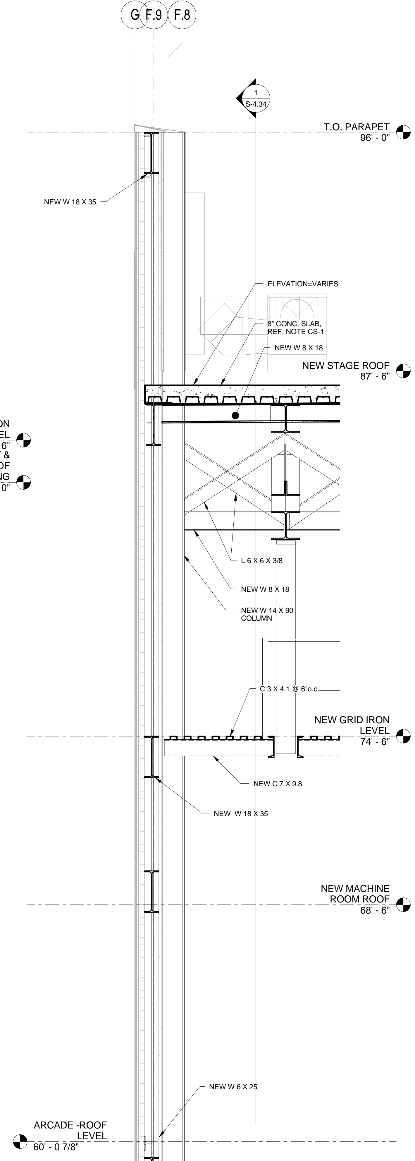
3 SECTION 1/2" = 1'-0"
