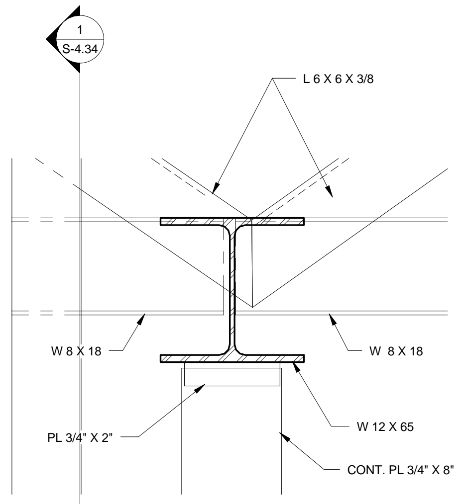
4 DETAIL 1 1/2" = 1'-0"
