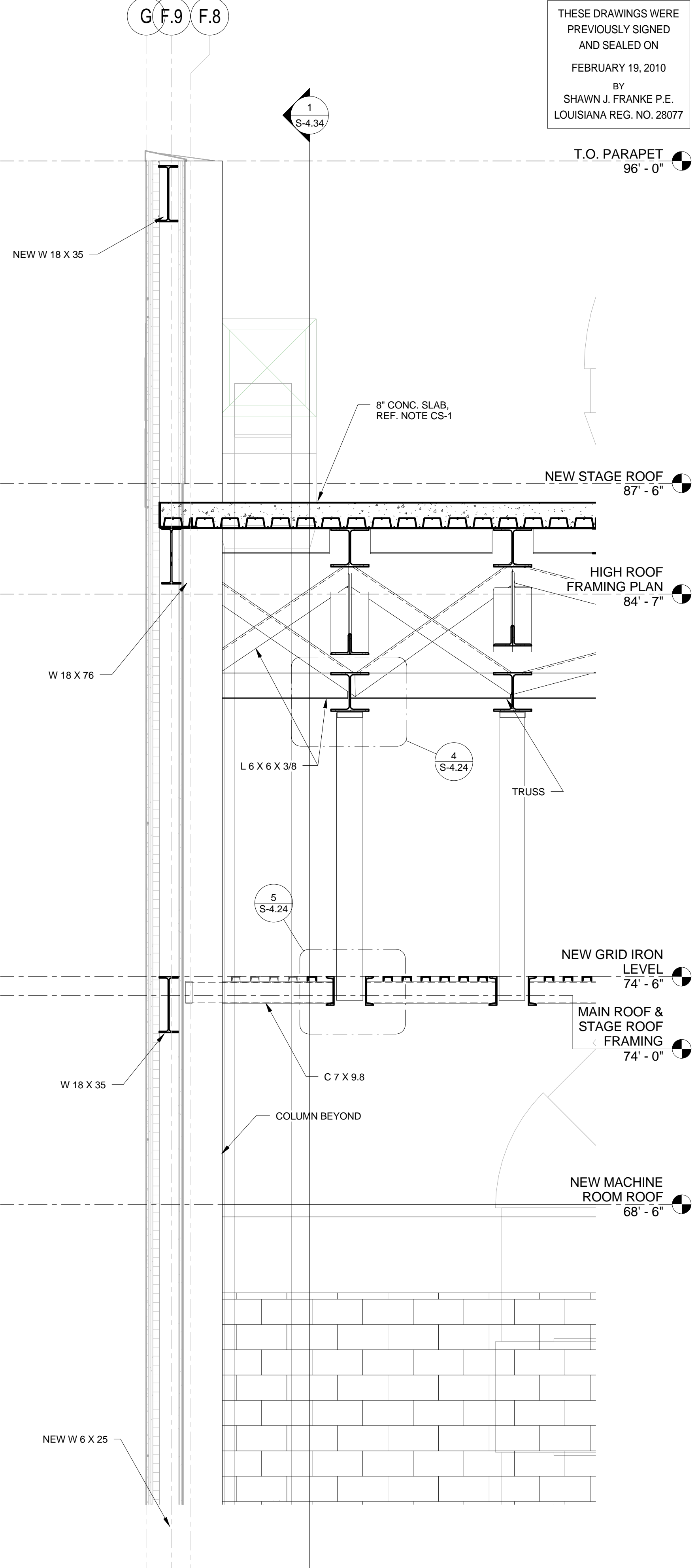
1 SECTION 1/2" = 1'-0"
