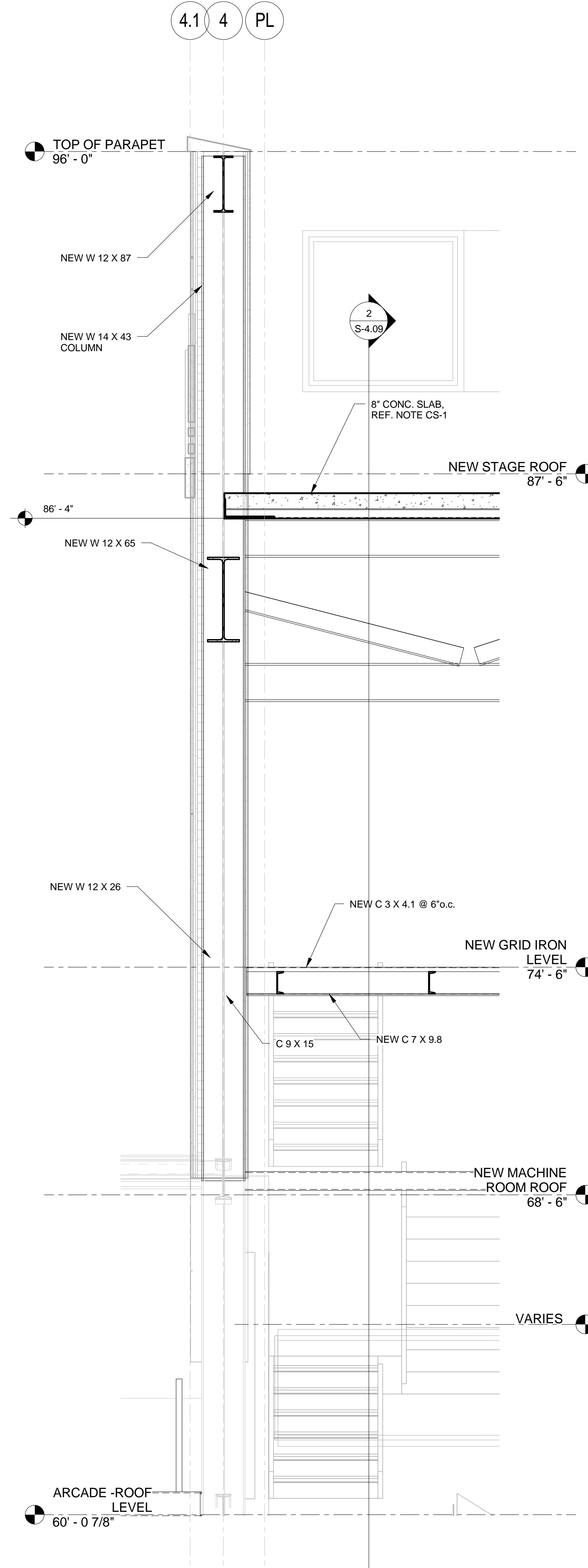
2 SECTION 1/2" = 1'-0"
