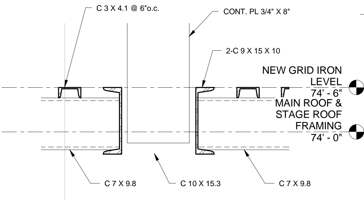
4 DETAIL 1 1/2" = 1'-0"
