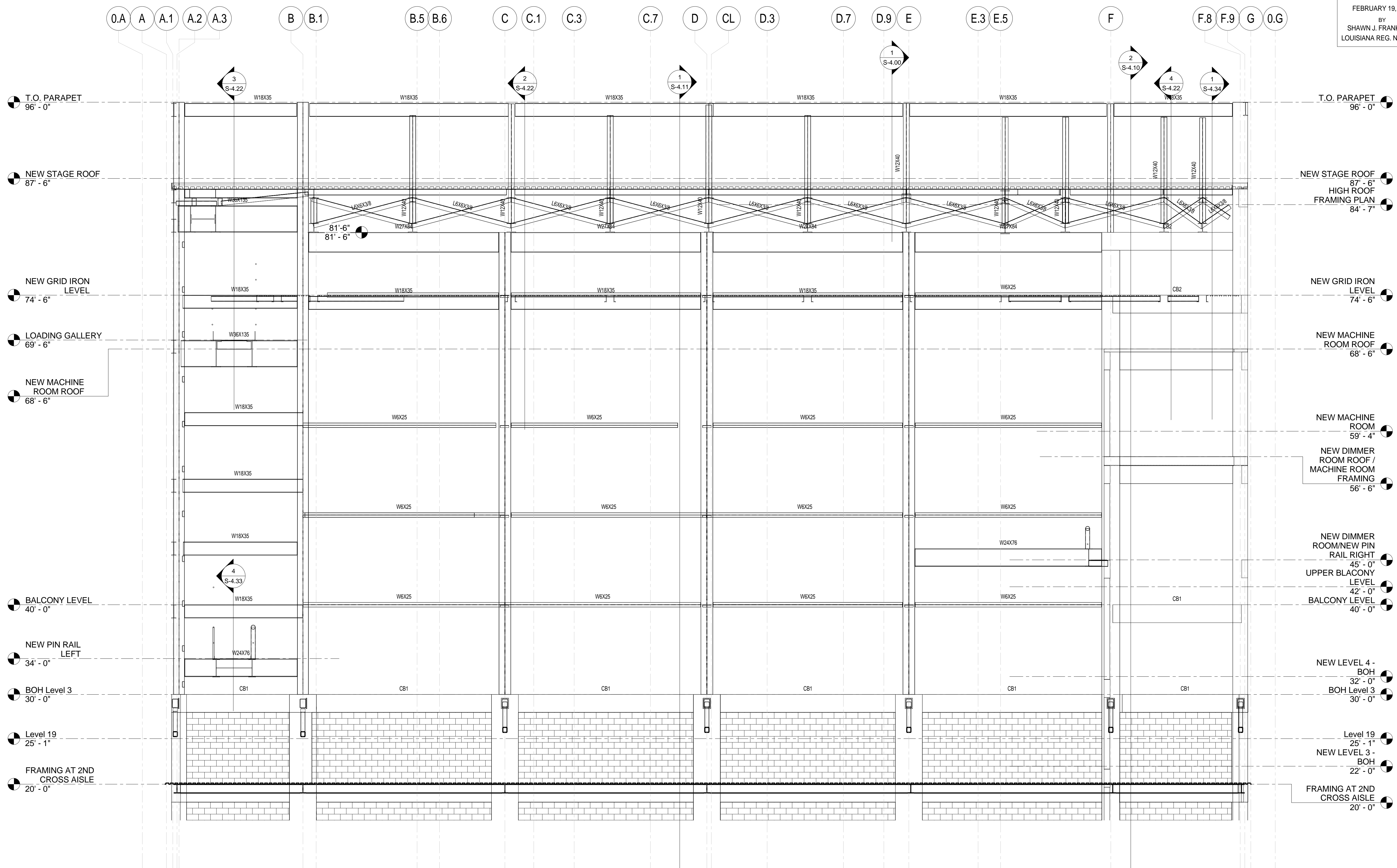
1 SECTION 3/16" = 1'-0"
