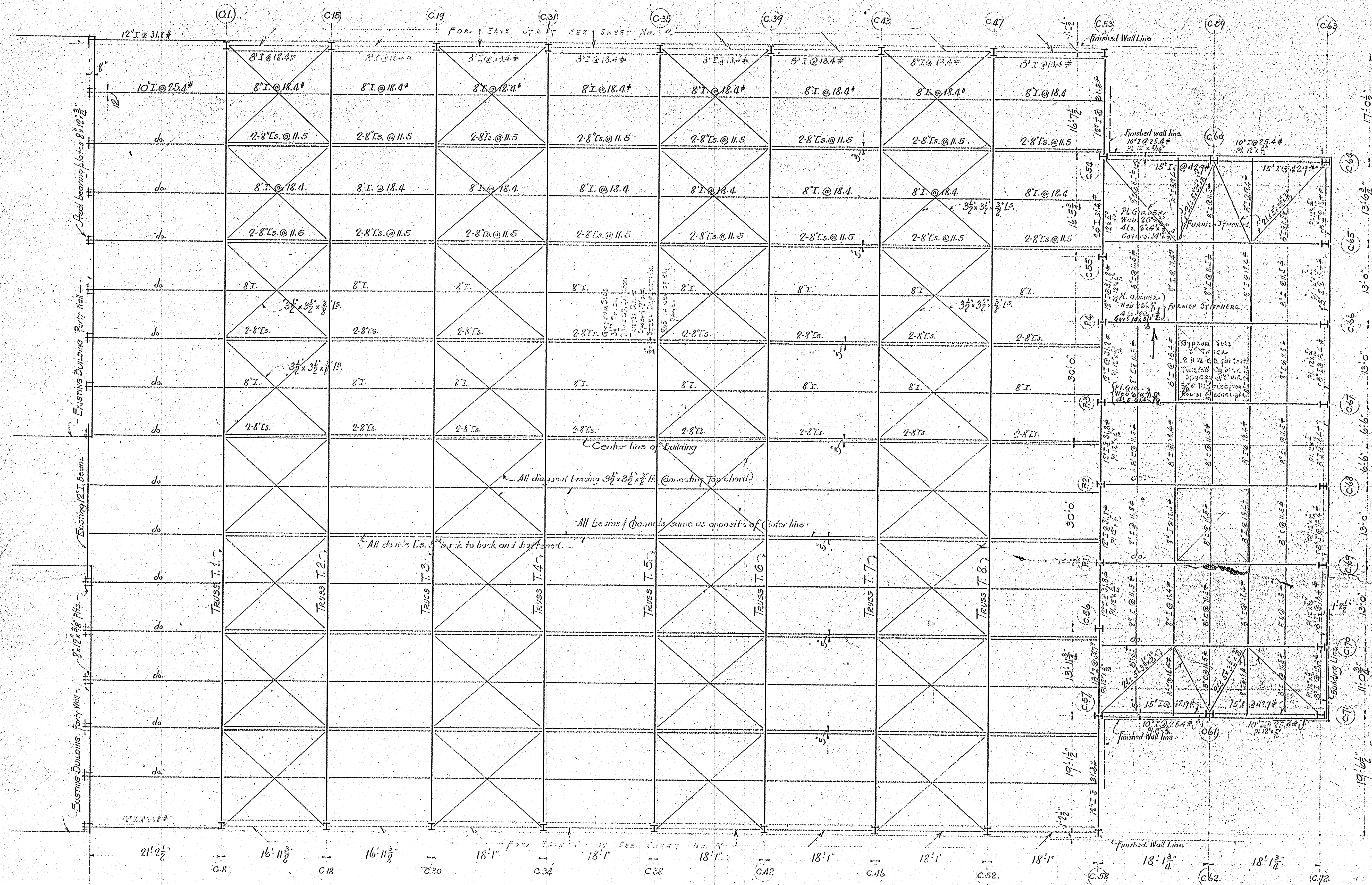
MAIN ROOF & STAGE ROOF FRAMING SCALE 1/8" = 1'-0"
