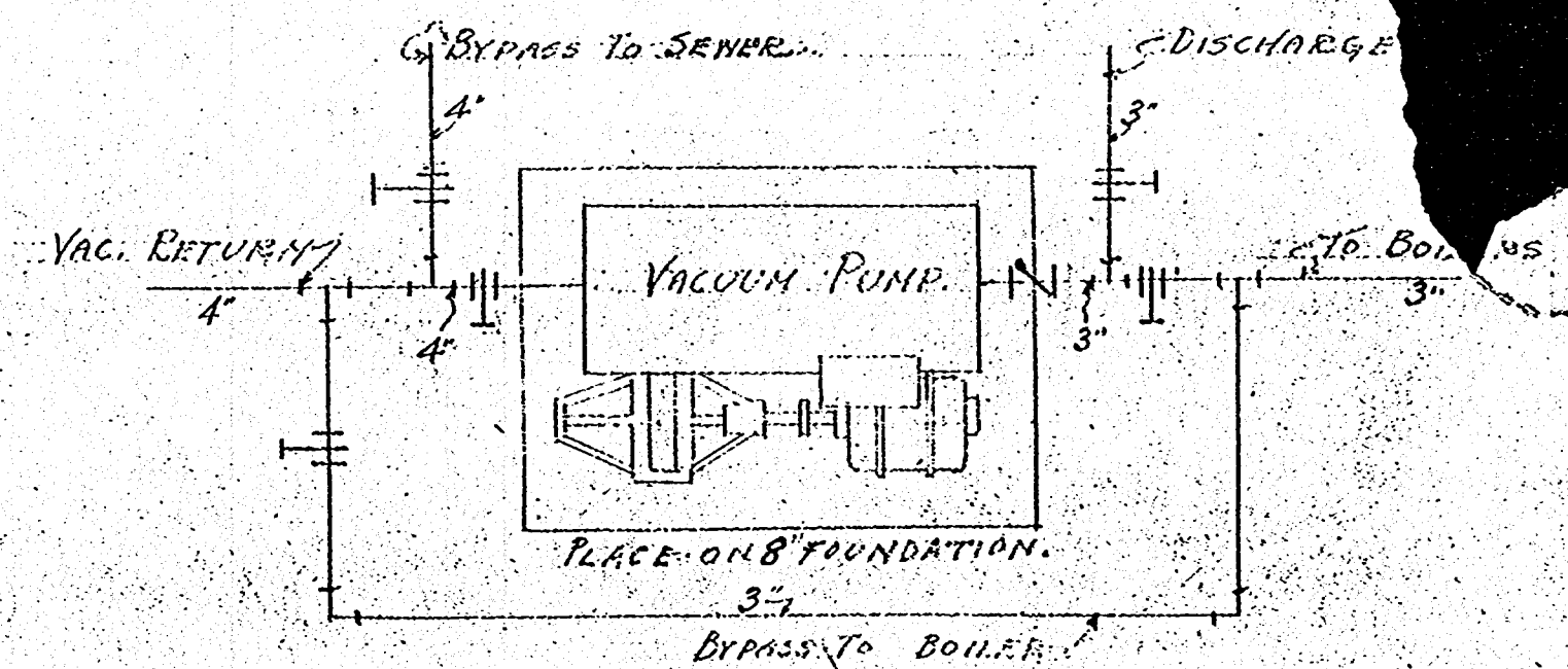
DETAIL OF CONNECTIONS AROUND VACUUM PUMP NO SCALE
