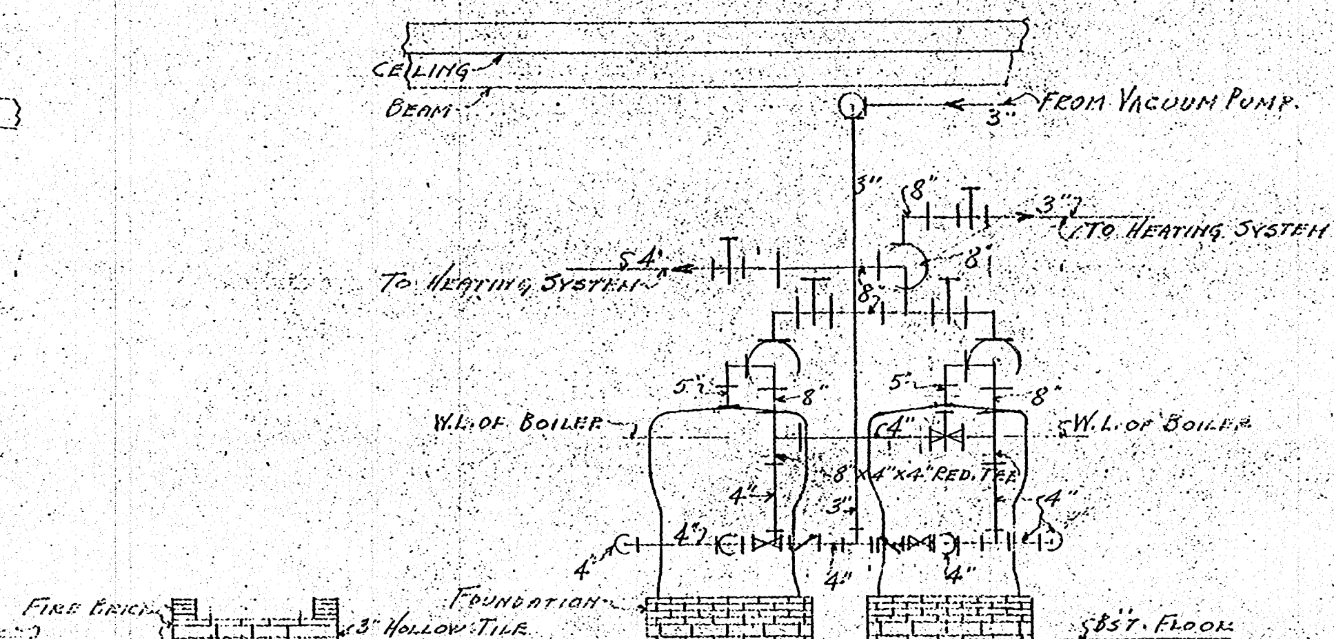
SECTION SHOWING BOILER FOUNDATIONS SCALE: 1/4" = 1'-0"
