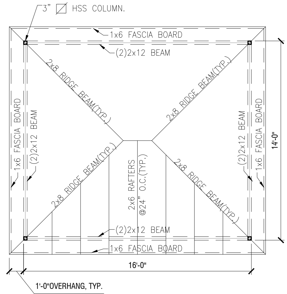
1 GAZEBO PLOT PLAN Scale: 1/4"=1'-0"
