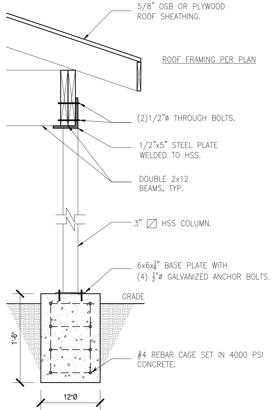
2 GAZEBO FOUNDATION & FRAMING SECTION Scale: 1"=1'-0"
