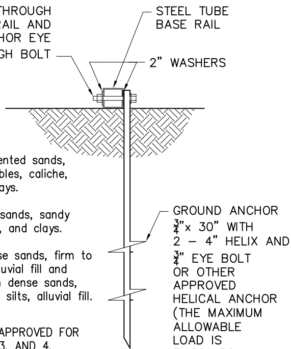
1 SOIL BASE RAIL ANCHOR DETAIL
