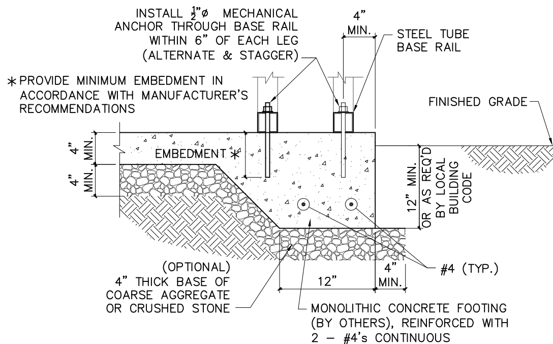
2 CONCRETE BASE RAIL ANCHORAGE (LADDER LEG)
