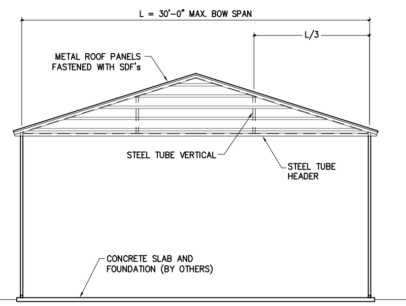
GABLE END ELEVATION
