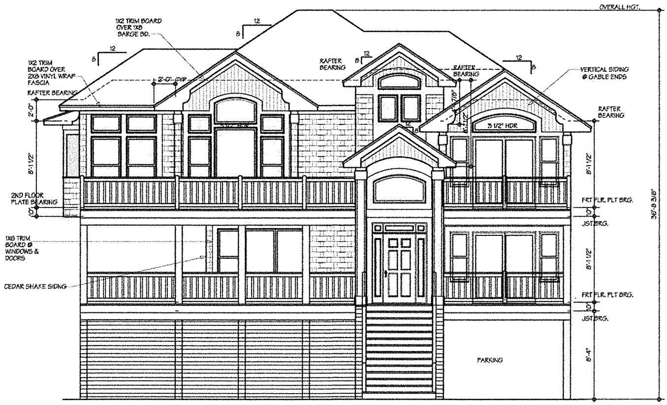
FRONT ELEVATION
