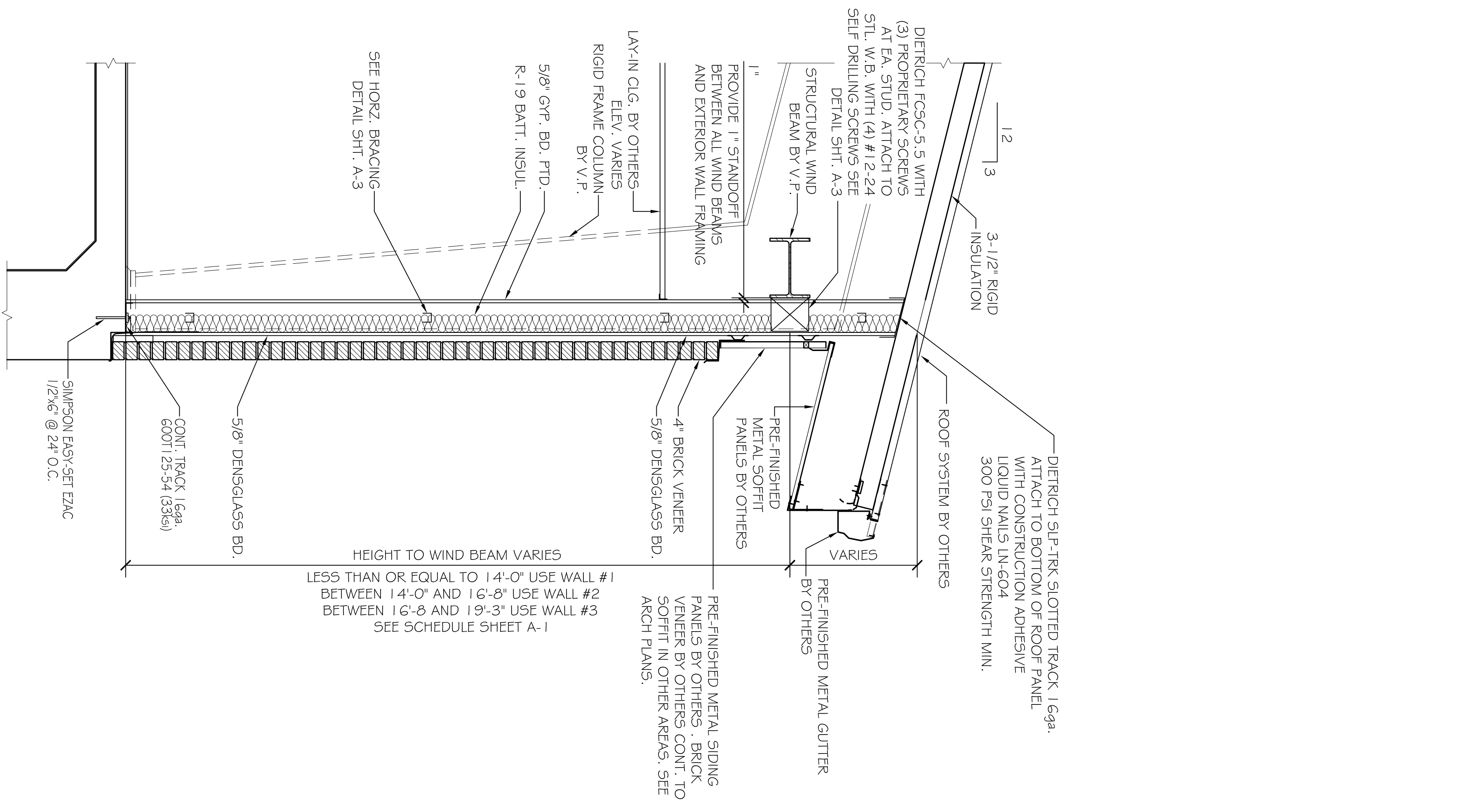
SIDE WALL DETAIL SCALE: 3/4" = 1'-0"
