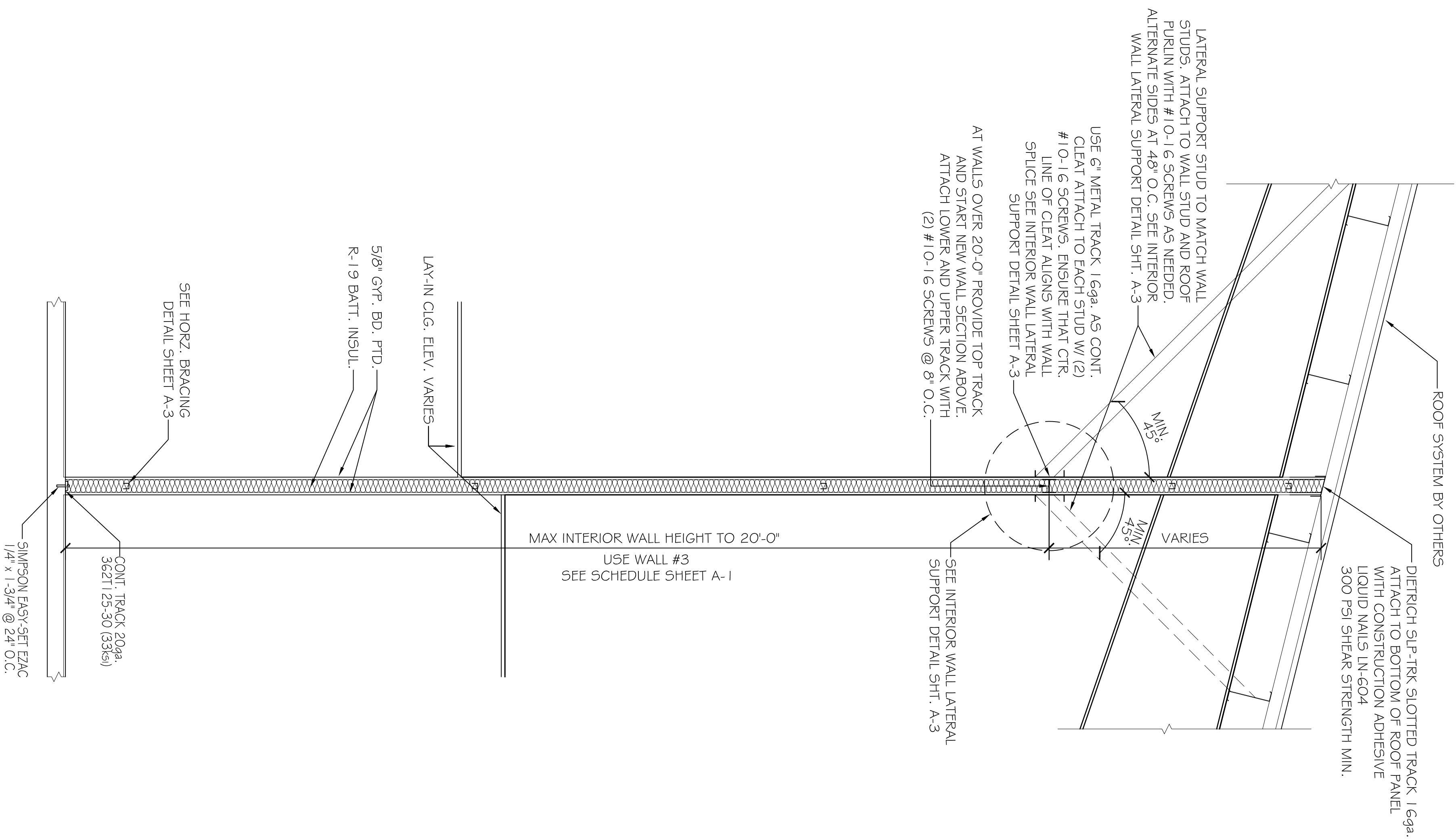
INTERIOR WALL DETAIL SCALE: 3/4" = 1'-0"
