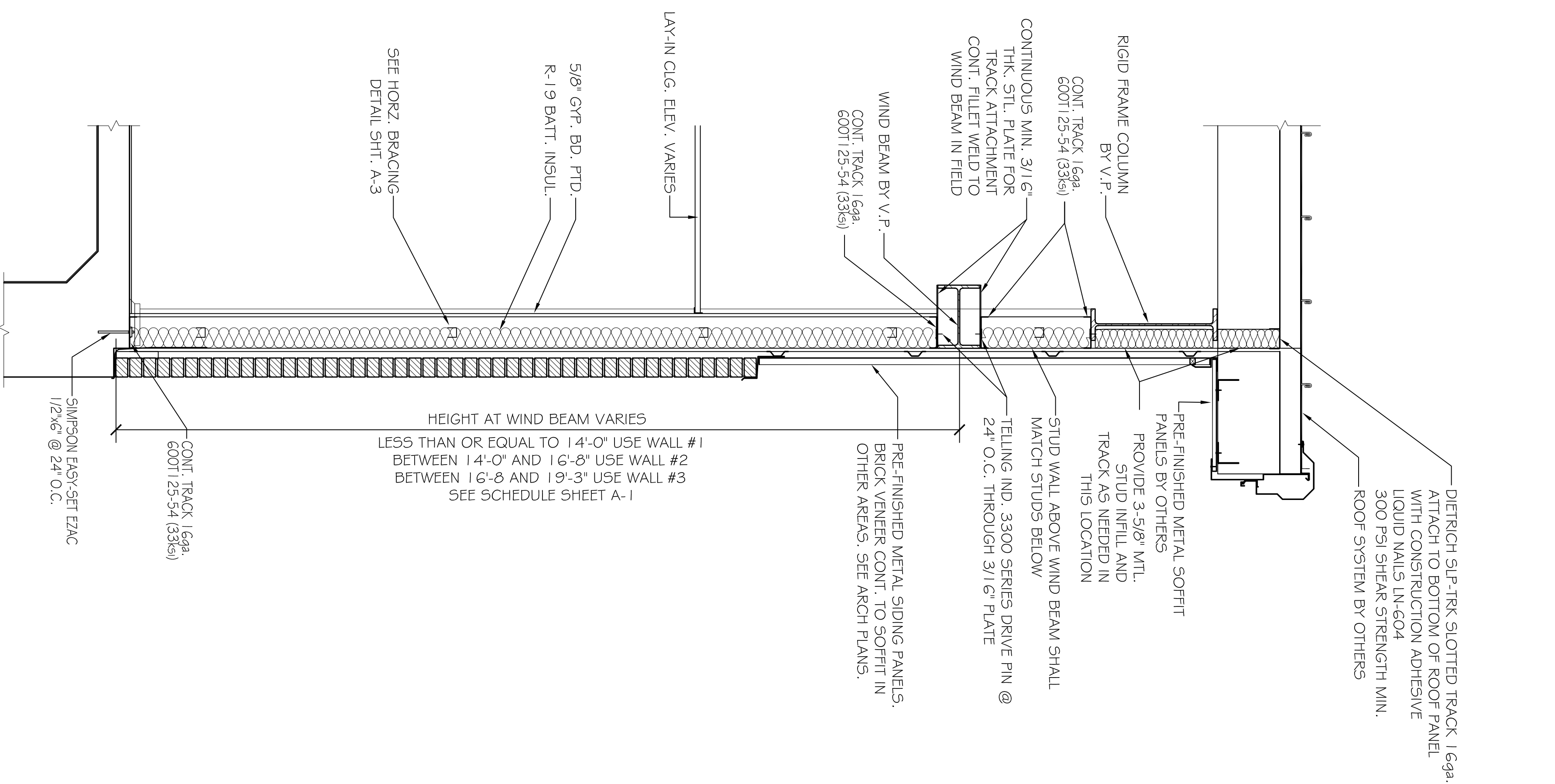
ENDWALL WALL DETAIL SCALE: 3/4" = 1'-0"
