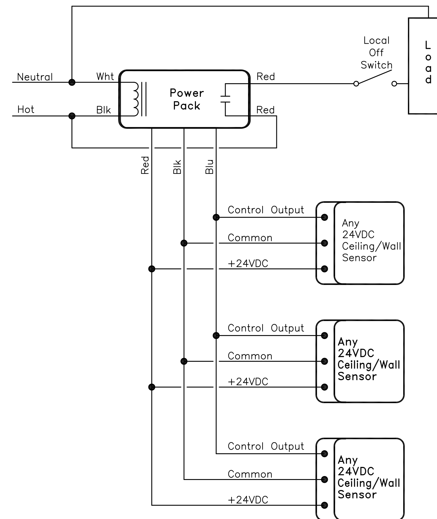
2 MULTIPLE OCCUPANCY SENSORS WIRING DIAGRAM SCALE: NONE
