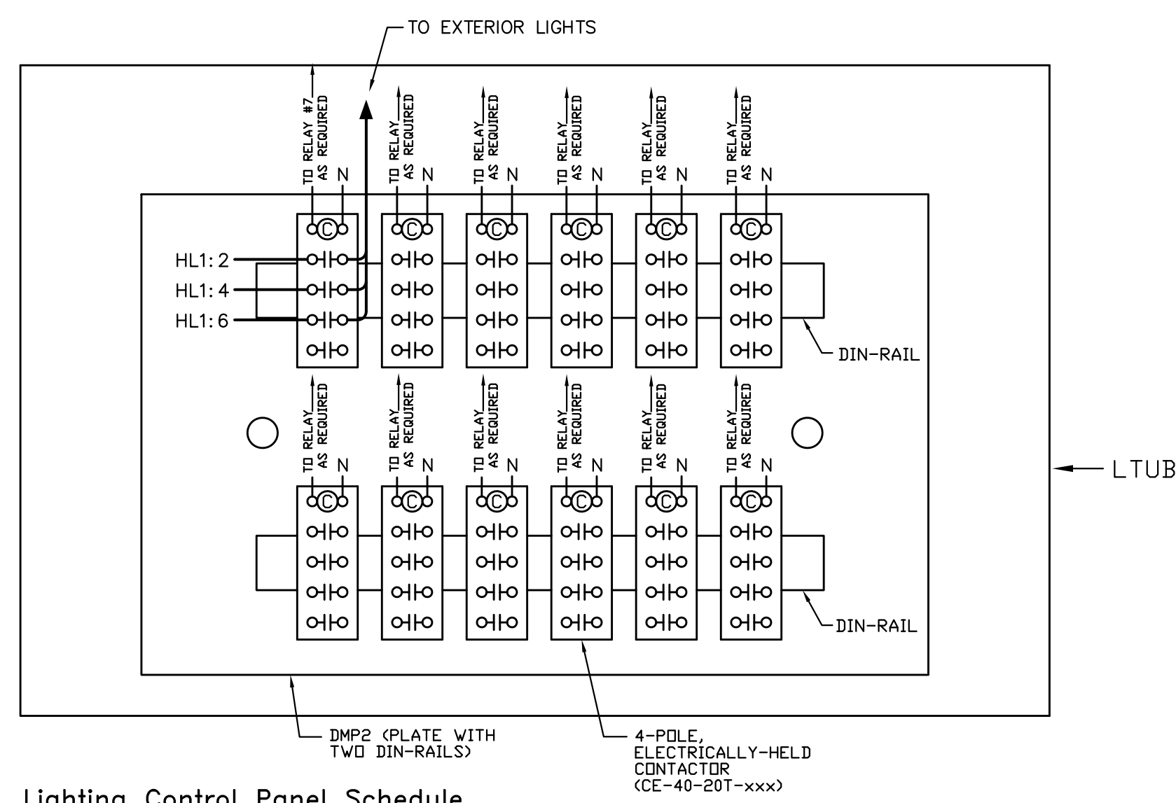
Lighting Control Panel Schedule
