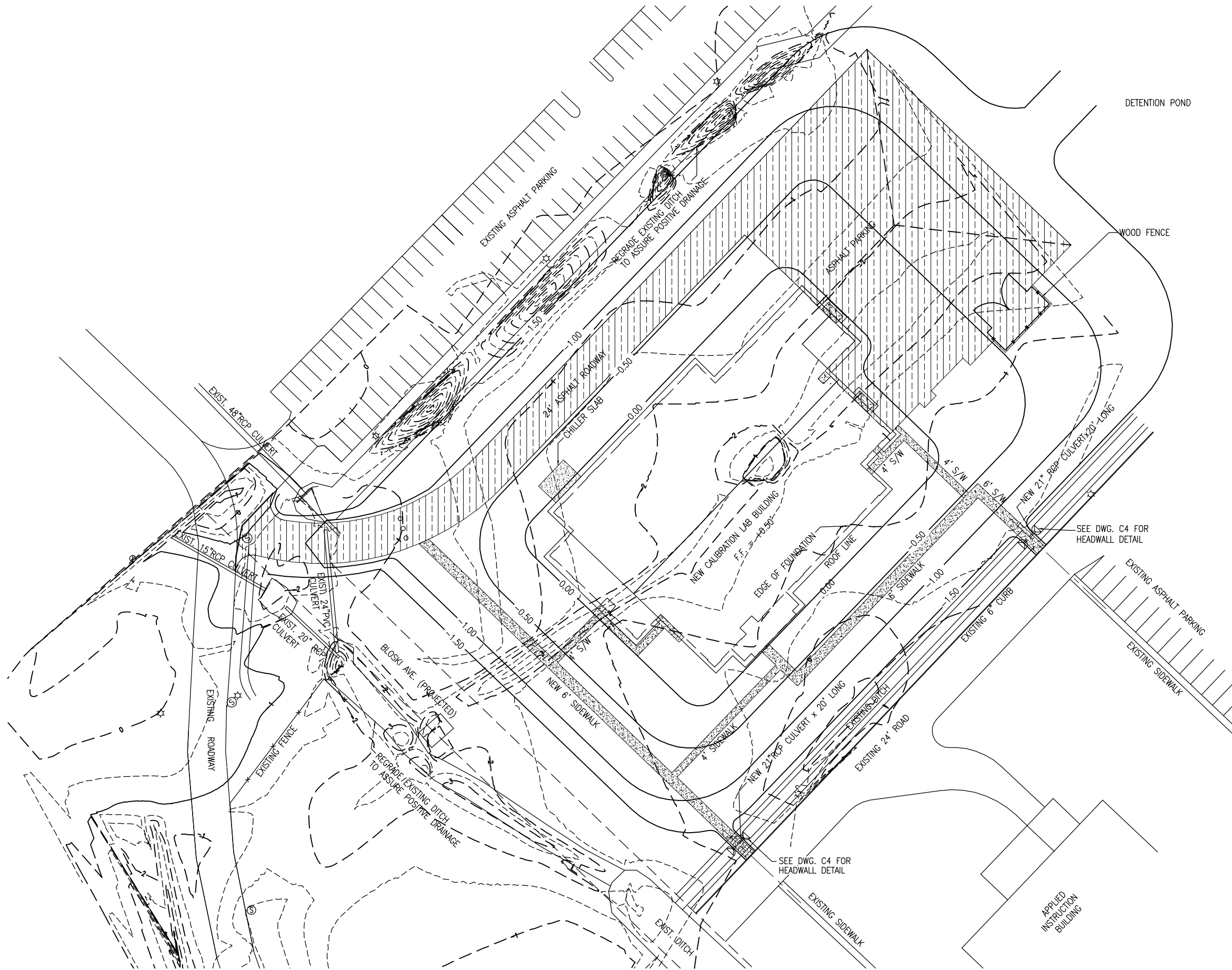
GRADING AND DRAINAGE PLAN
