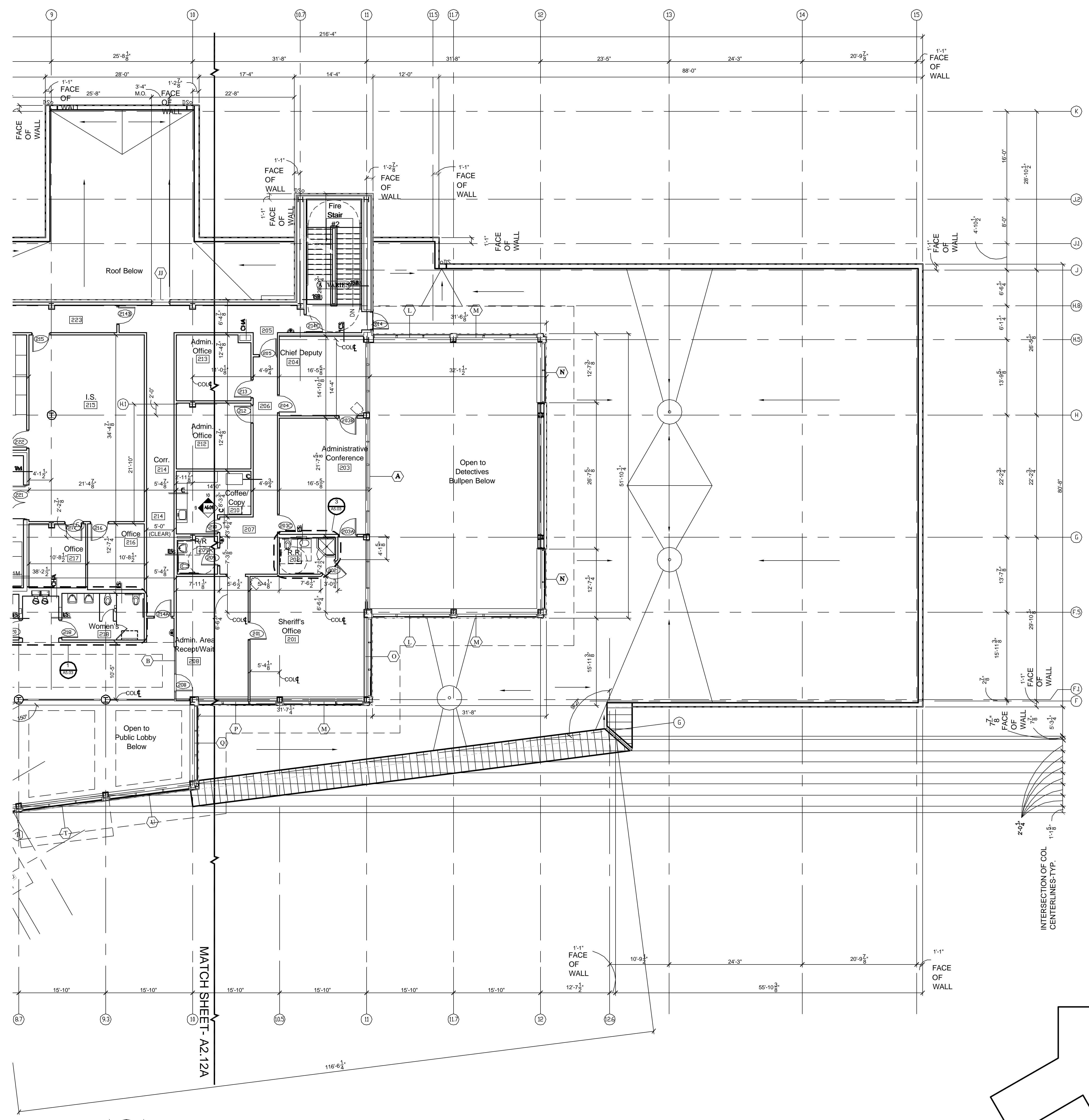
NORTH 1 2ND FLOOR DIMENSION PLAN "B" A2.12B 1/8"=1'-0"
