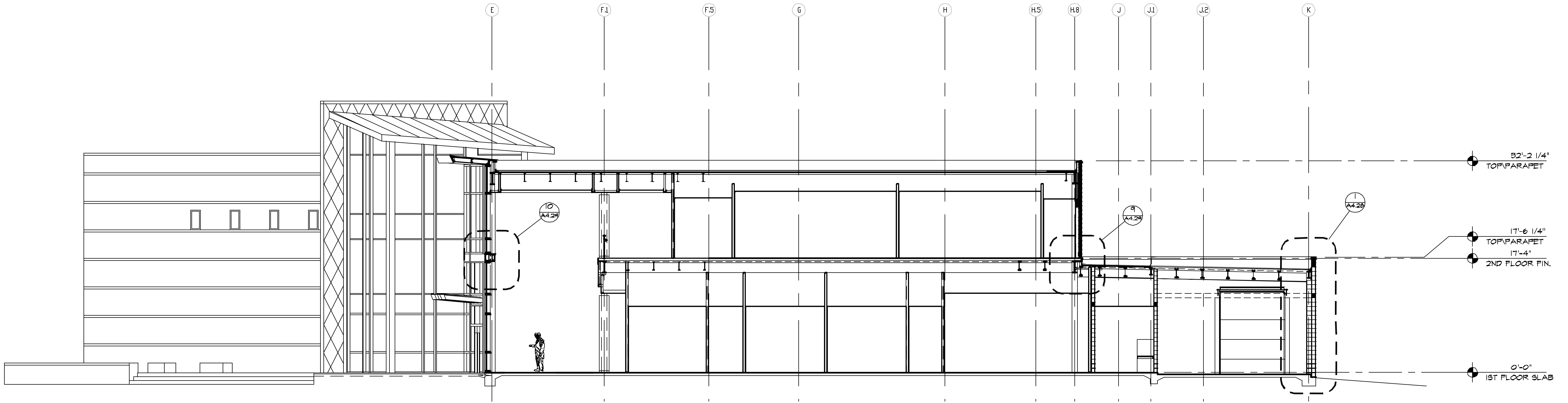
1 TRANSVERSE BUILDING SECTION A4.25 / 1/8"=1'-0"
