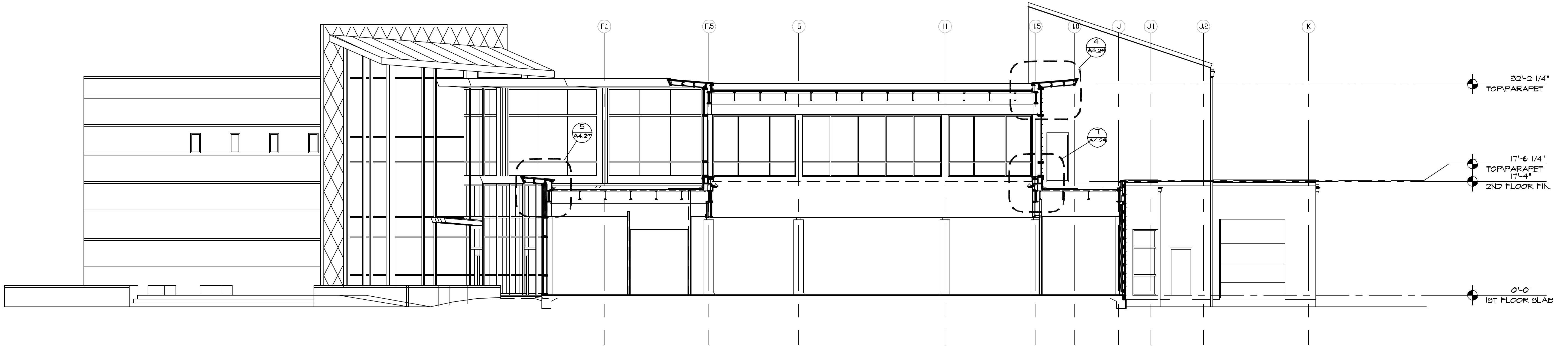
2 TRANSVERSE BUILDING SECTION A4.25 / 1/8"=1'-0"
