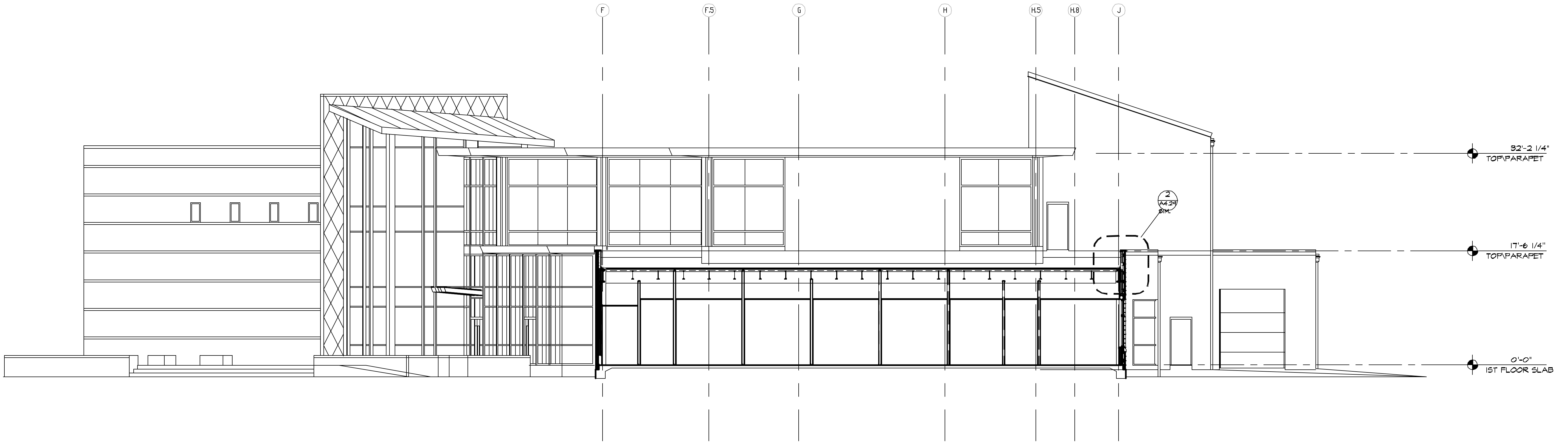
3 TRANSVERSE BUILDING SECTION A4.25 / 1/8"=1'-0"
