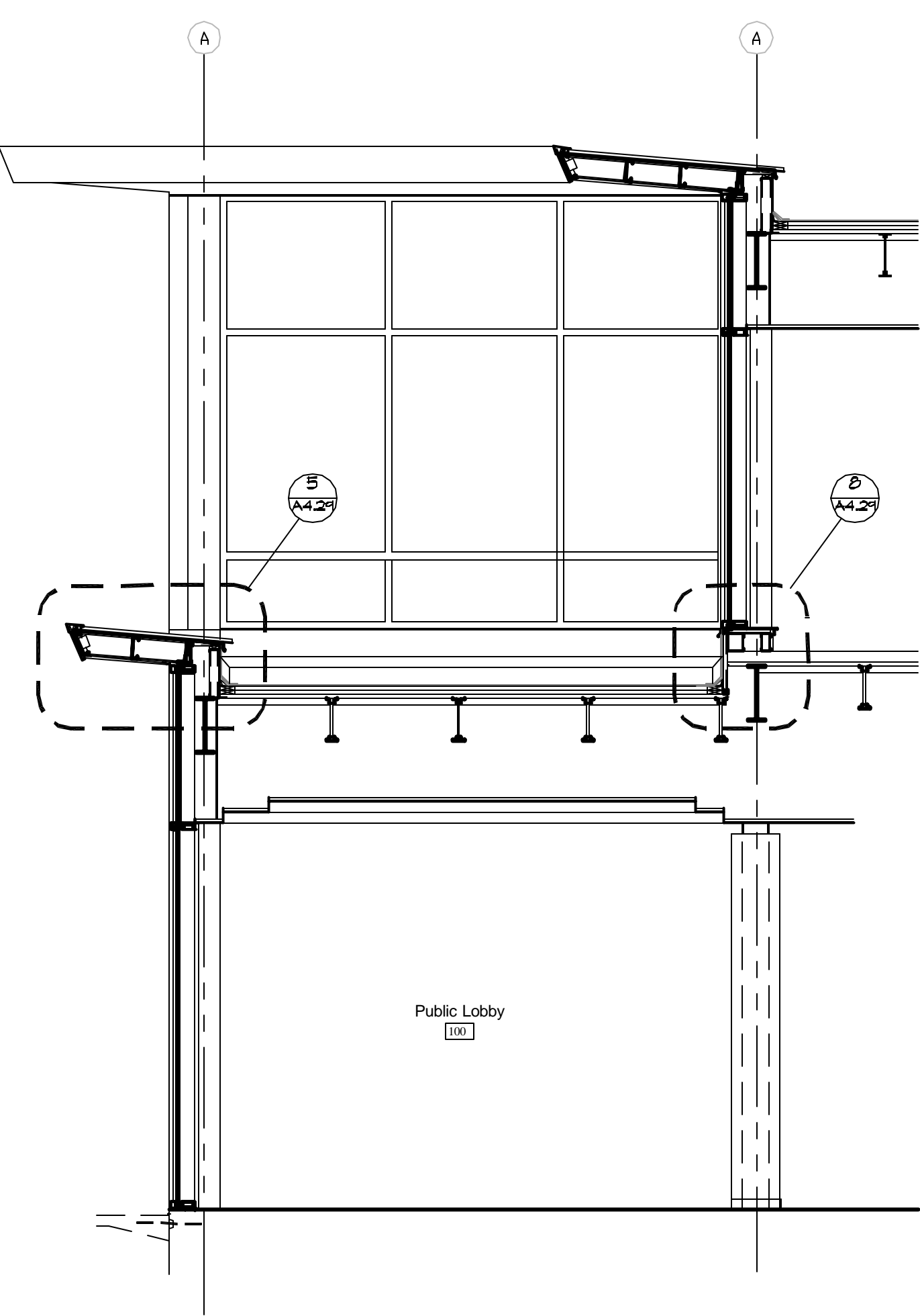
4 WALL SECTION A4.27 1/4"=1'-0"
