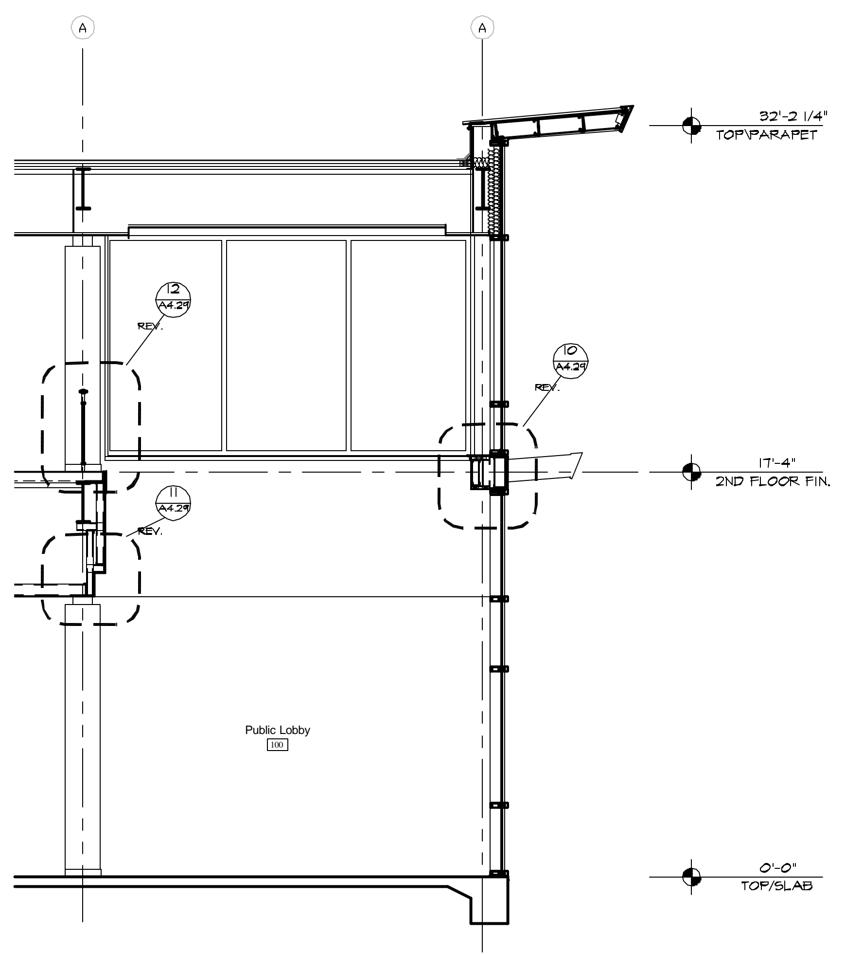
3 WALL SECTION A4.27 1/4"=1'-0"
