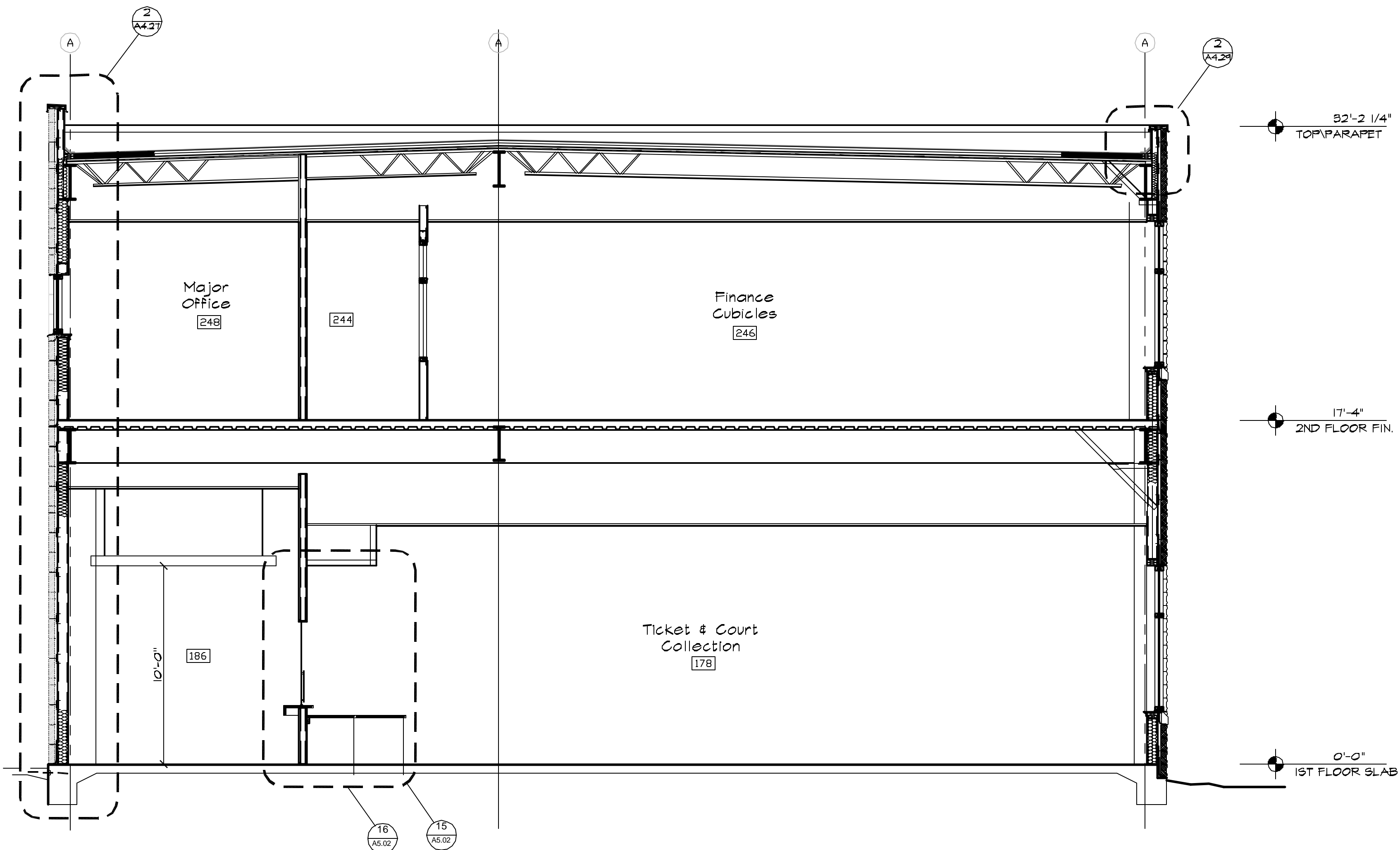
5 WALL SECTION A4.27 1/4"=1'-0"
