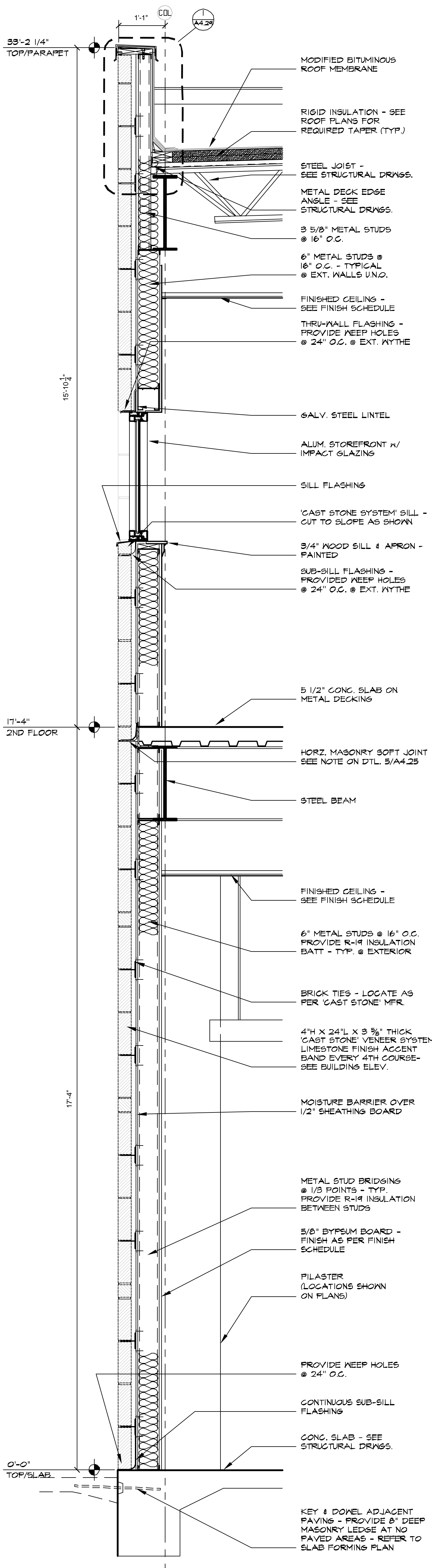
2 WALL SECTION A4.27 3/4"=1'-0"
