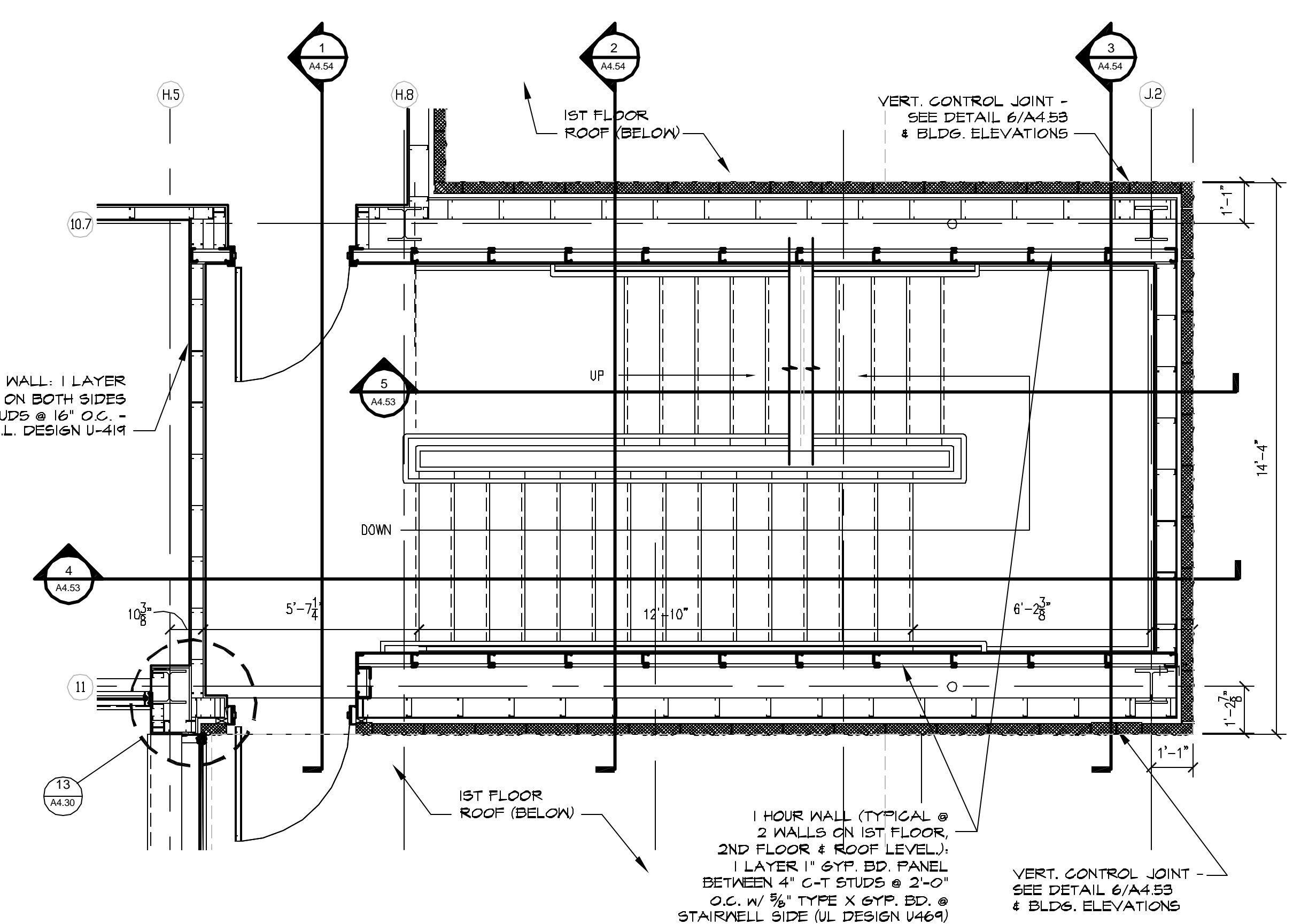
2 FIRE STAIR #2 PLAN - 2ND FLOOR SCALE: 3/8"=1'-0"
