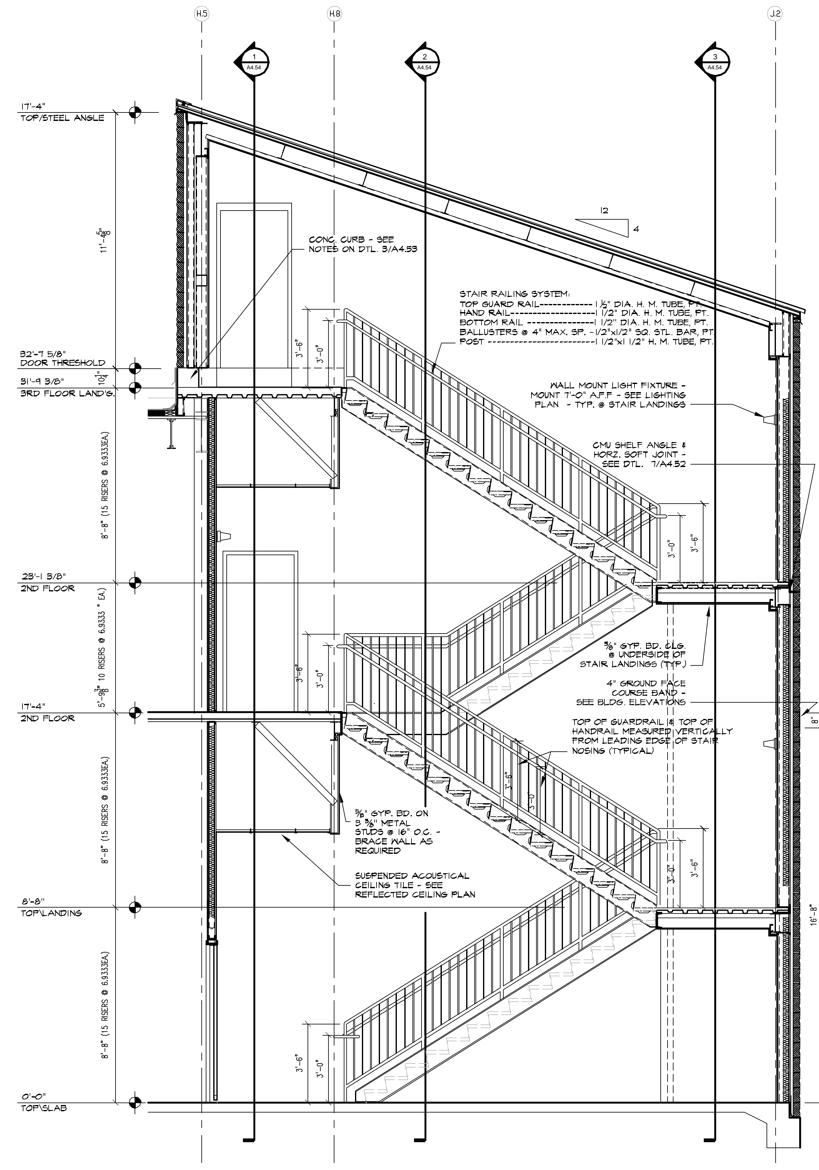
4 SECTION (FIRE STAIR #2) SCALE: 3/8"=1'-0"
