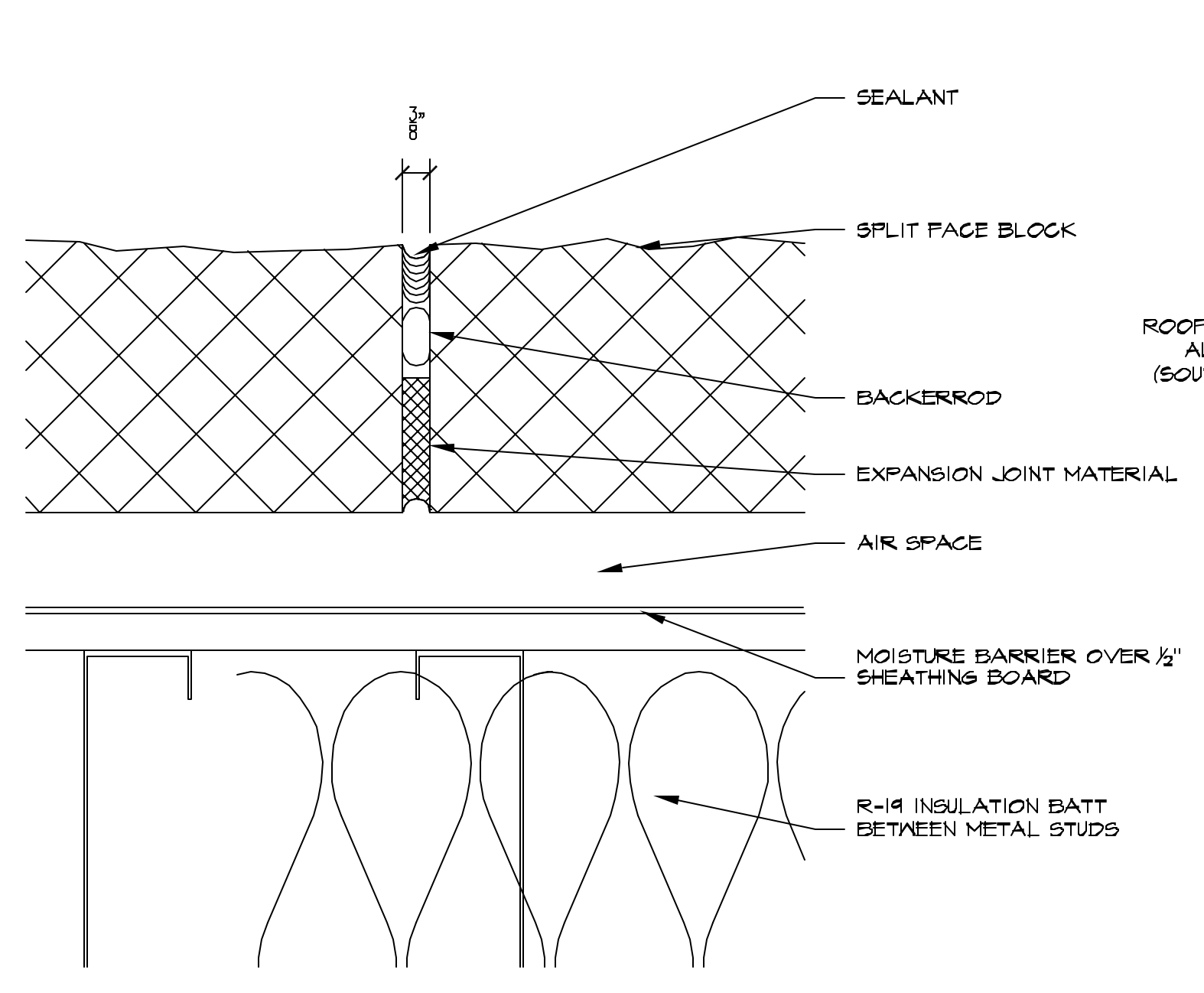
6 CMU VERTICAL CONTROL JOINT SCALE: 6"=1'-0"
