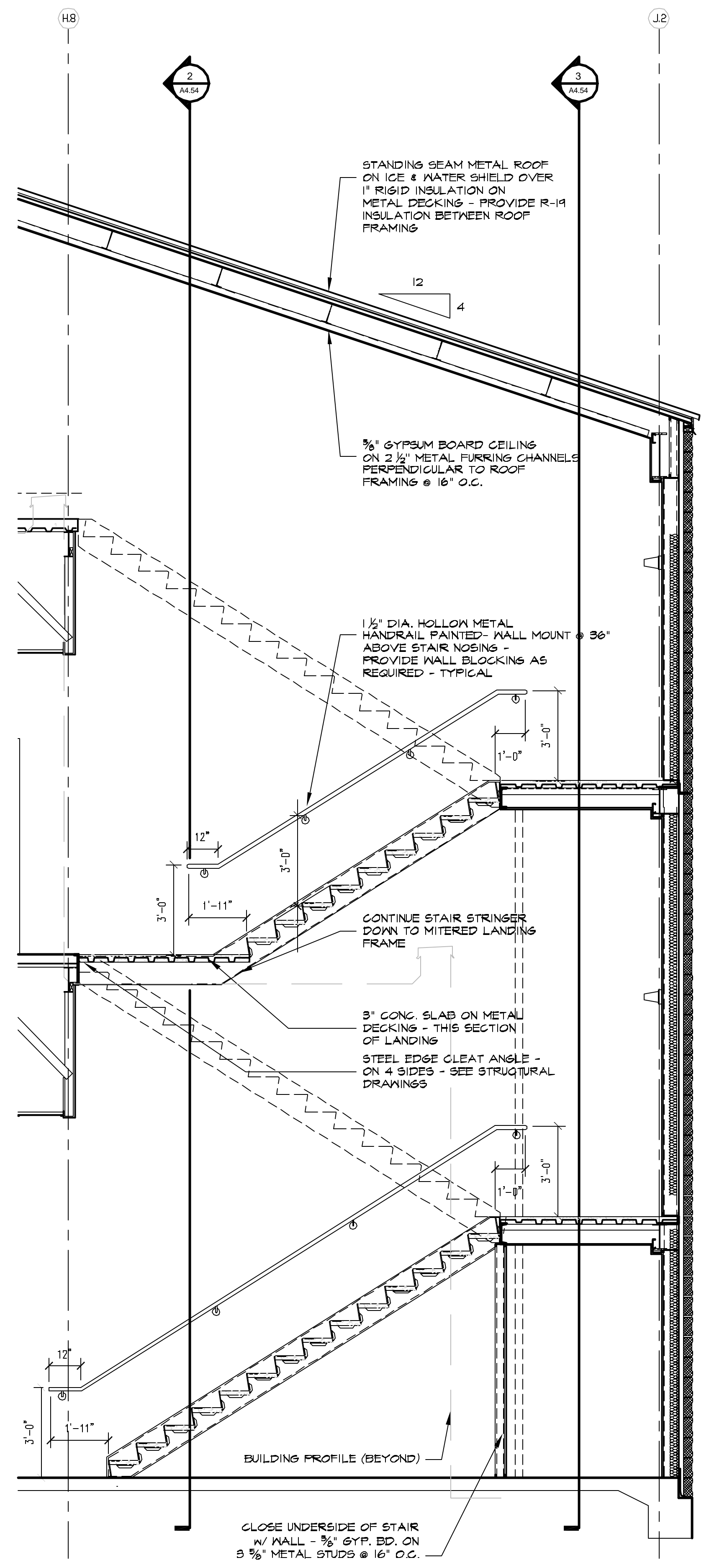
5 SECTION (FIRE STAIR #2) SCALE: 3/8"=1'-0"
