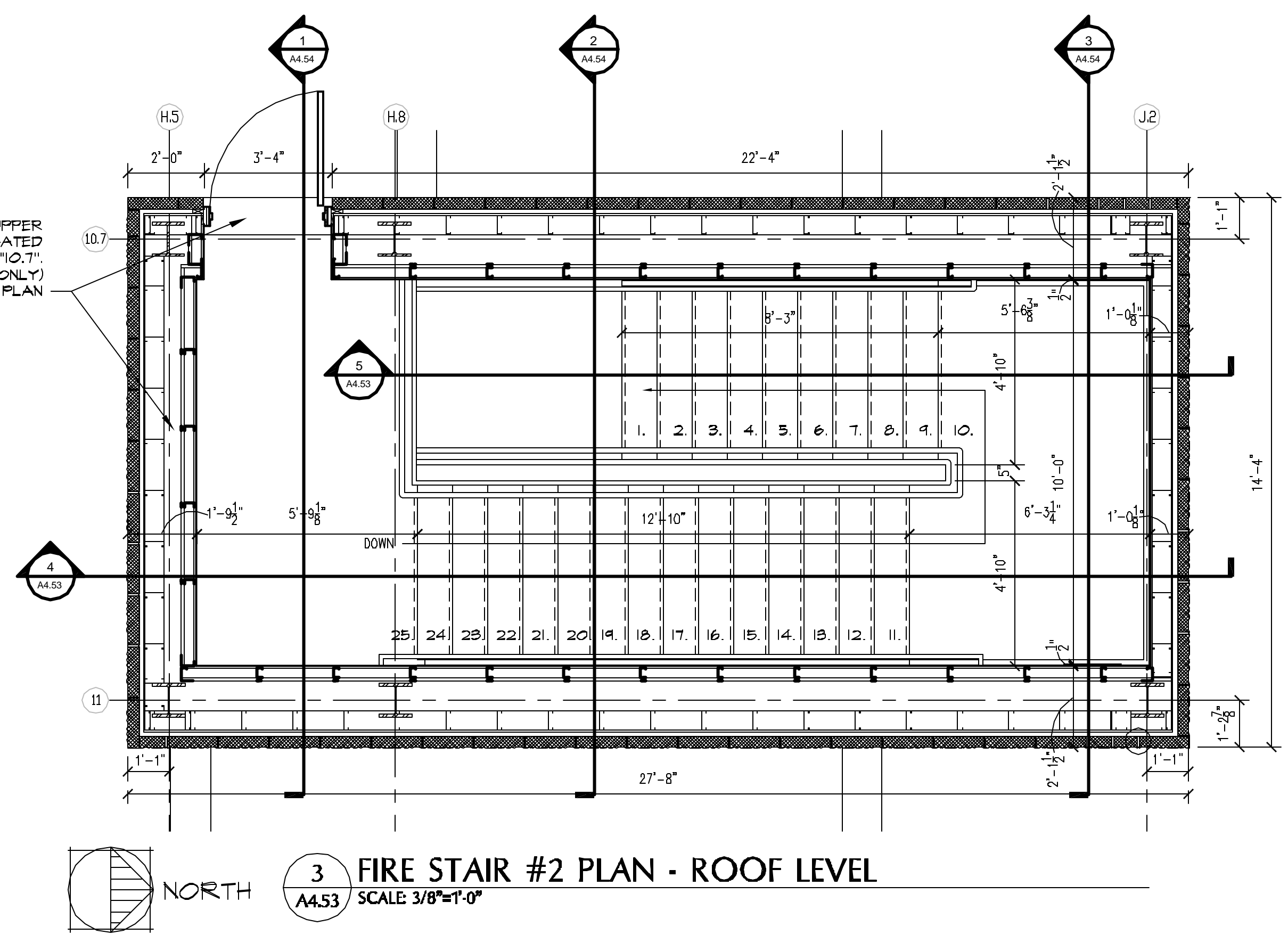
3 FIRE STAIR #2 PLAN - ROOF LEVEL SCALE: 3/8"=1'-0"
