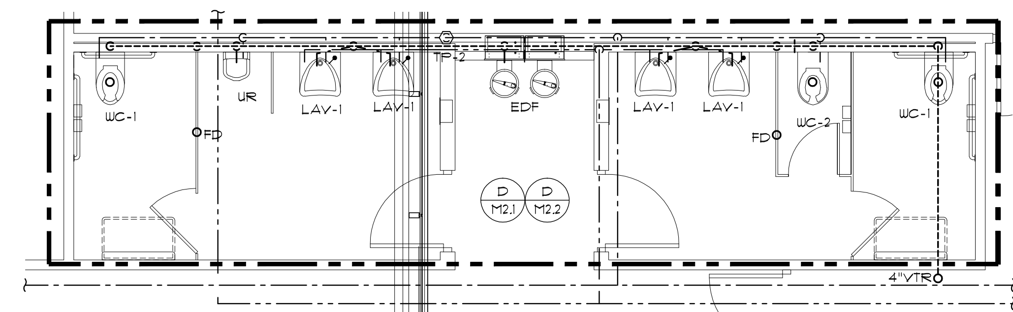
2 132 PUBLIC WOMEN'S R/R 134 PUBLIC MEN'S R/R 1/4" = 1'-0"
