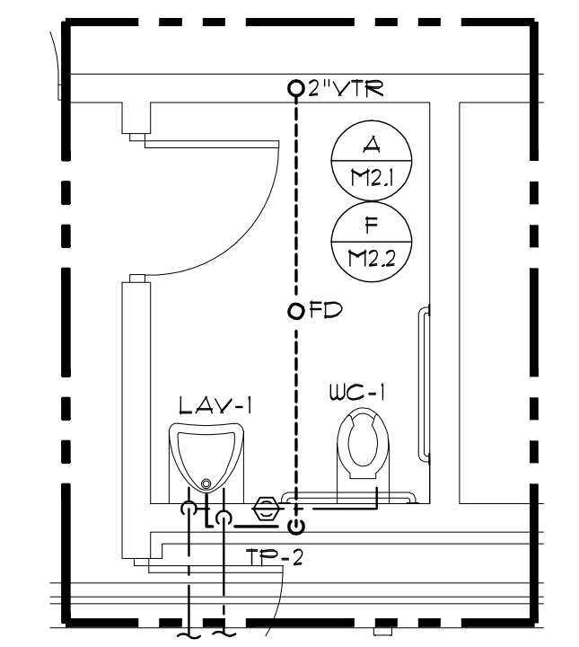
4 147 INTOX R/R 1/4" = 1'-0"
