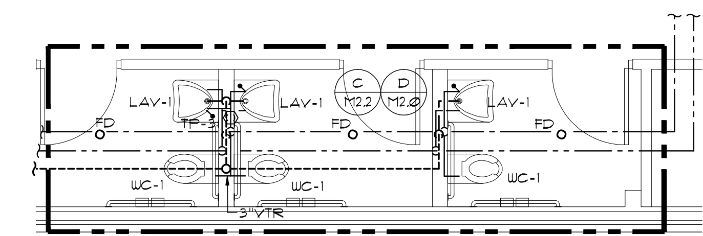
3 112 KIDS R/R 113 MEN R/R 114 WOMEN R/R 1/4" = 1'-0"
