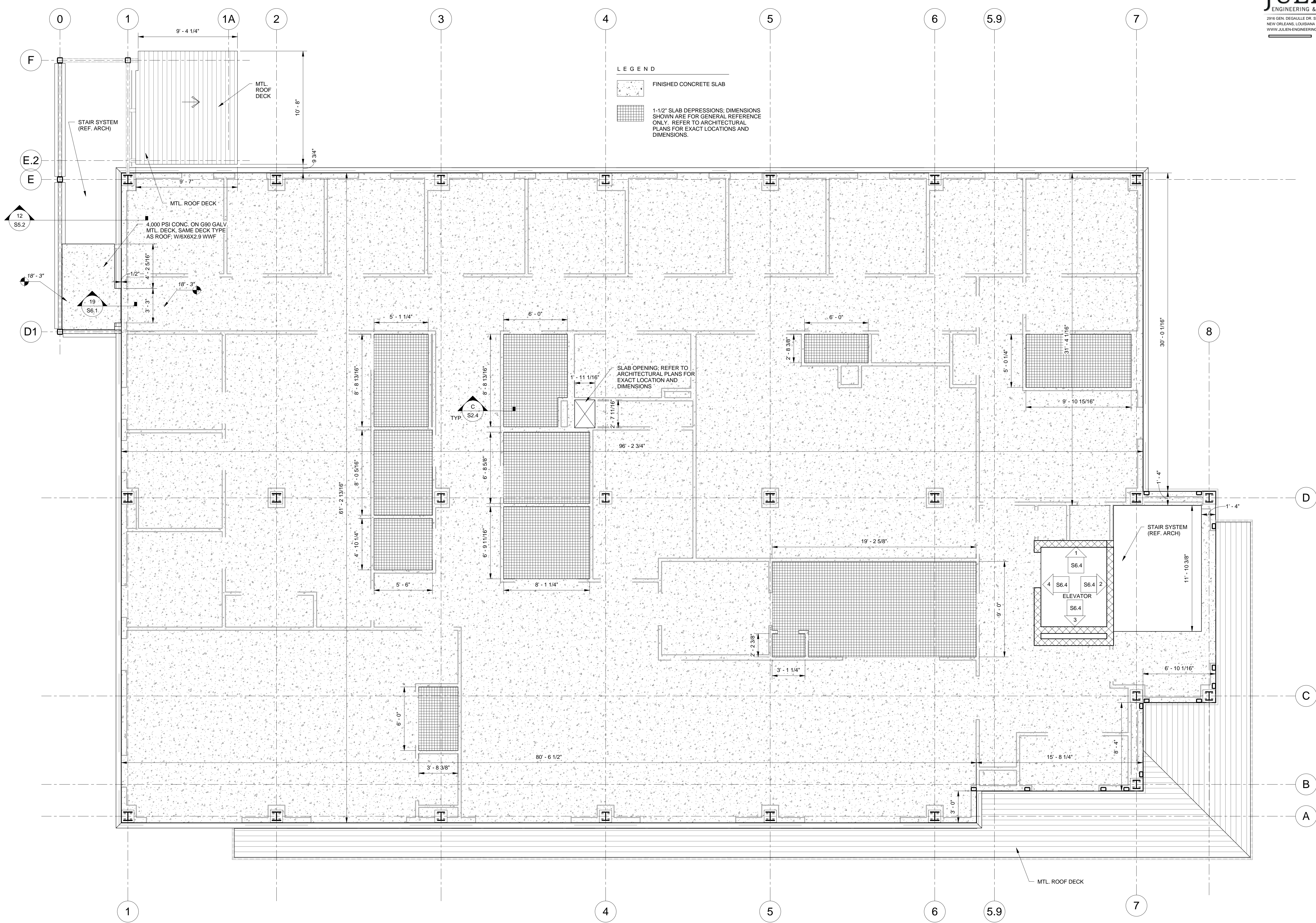
S2.2 - level 2 slab plan 1/4\"/>
