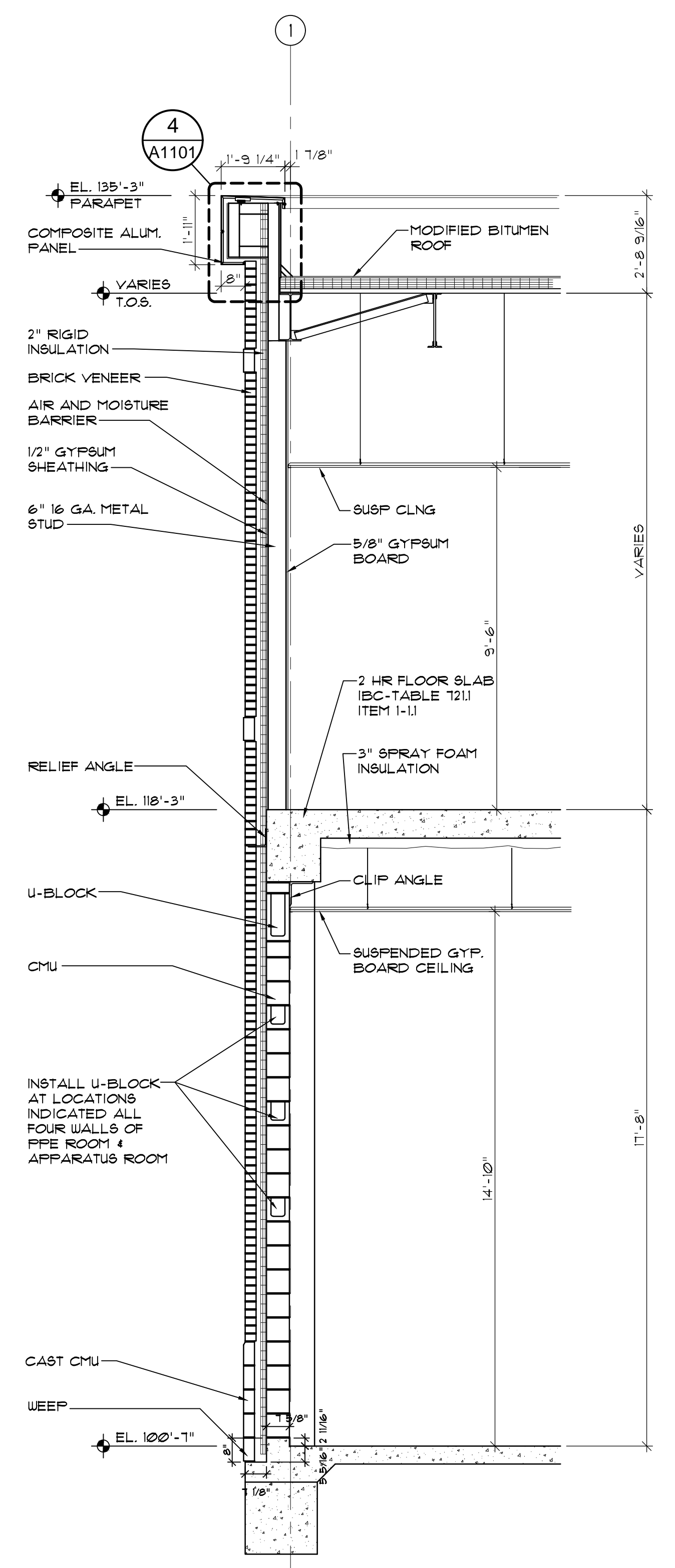
1 WALL SECTION A603 SCALE: 3/4" = 1'-0"
