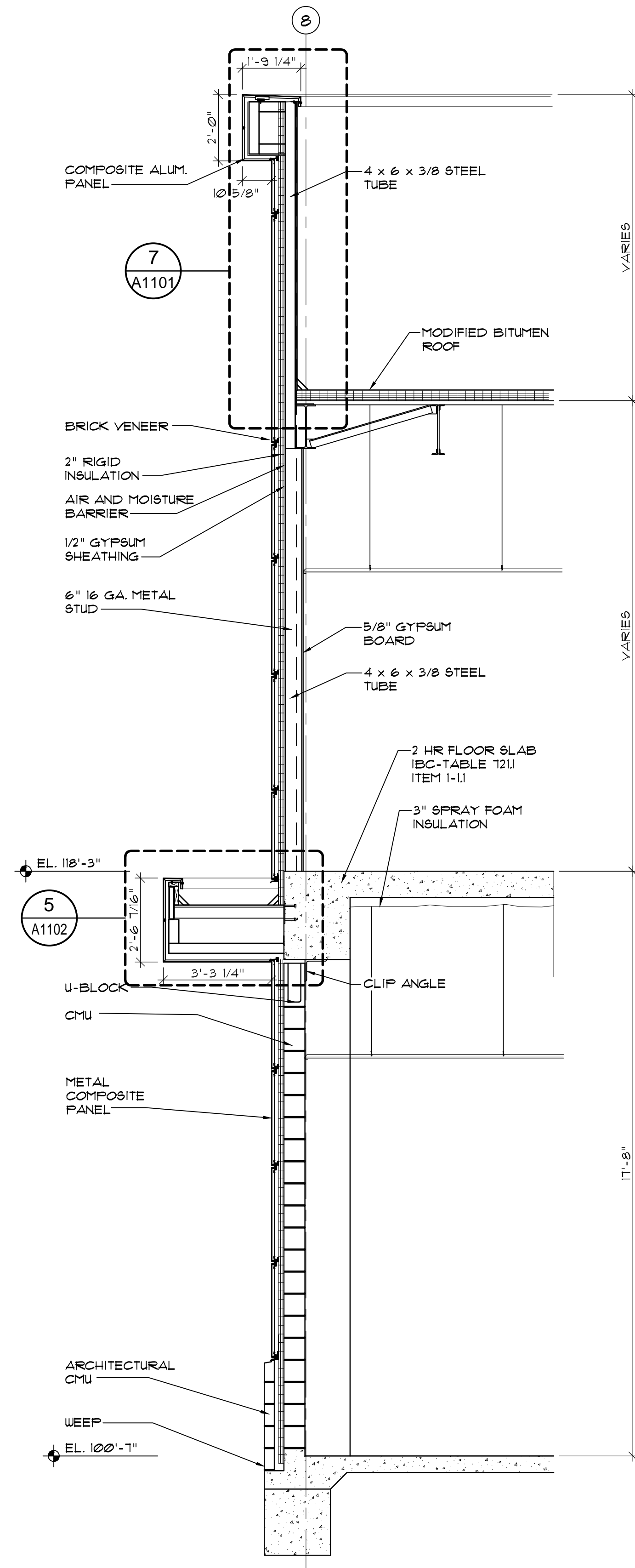
3 WALL SECTION A603 SCALE: 3/4" = 1'-0"
