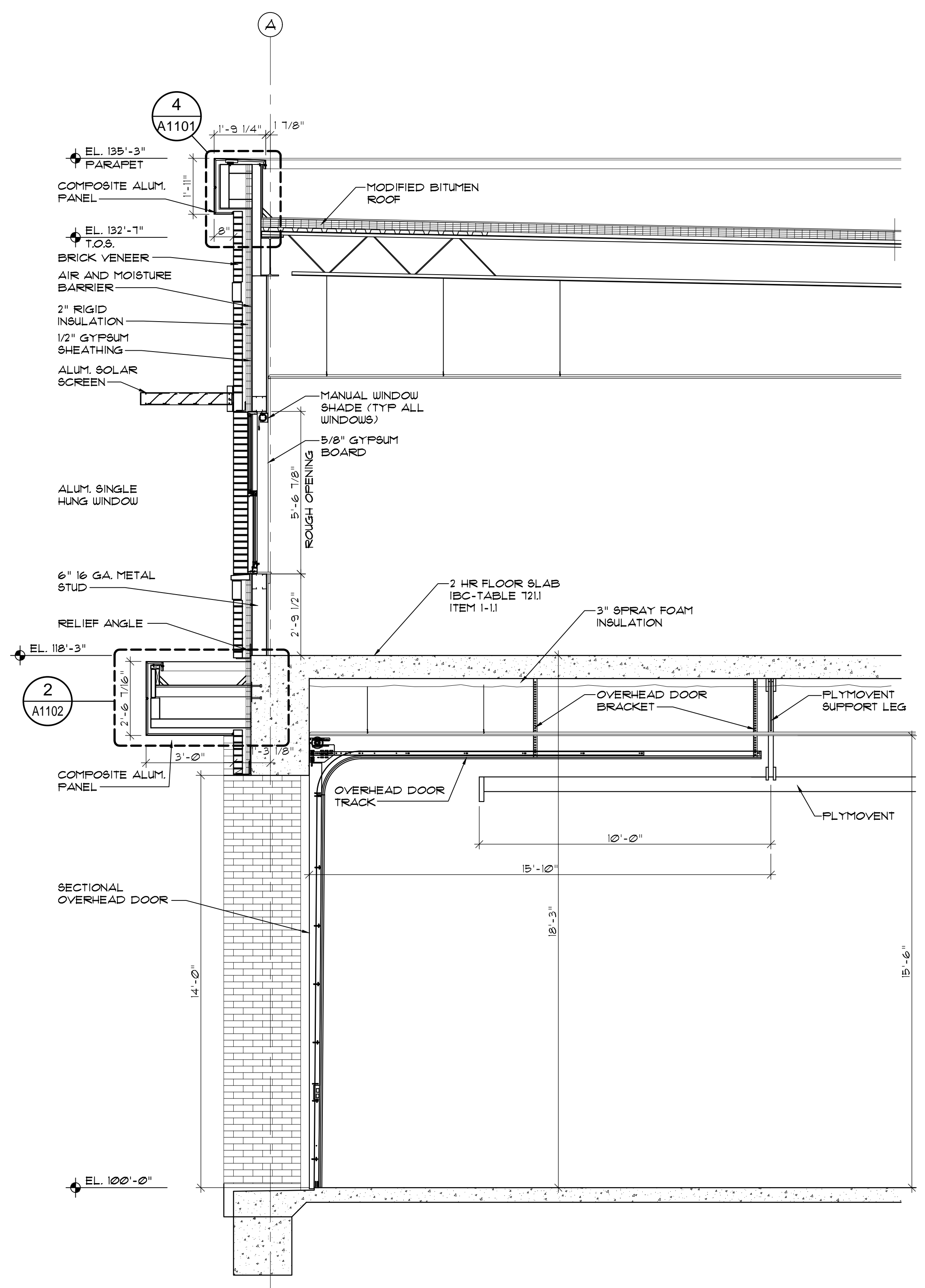
2 WALL SECTION A603 SCALE: 3/4" = 1'-0"
