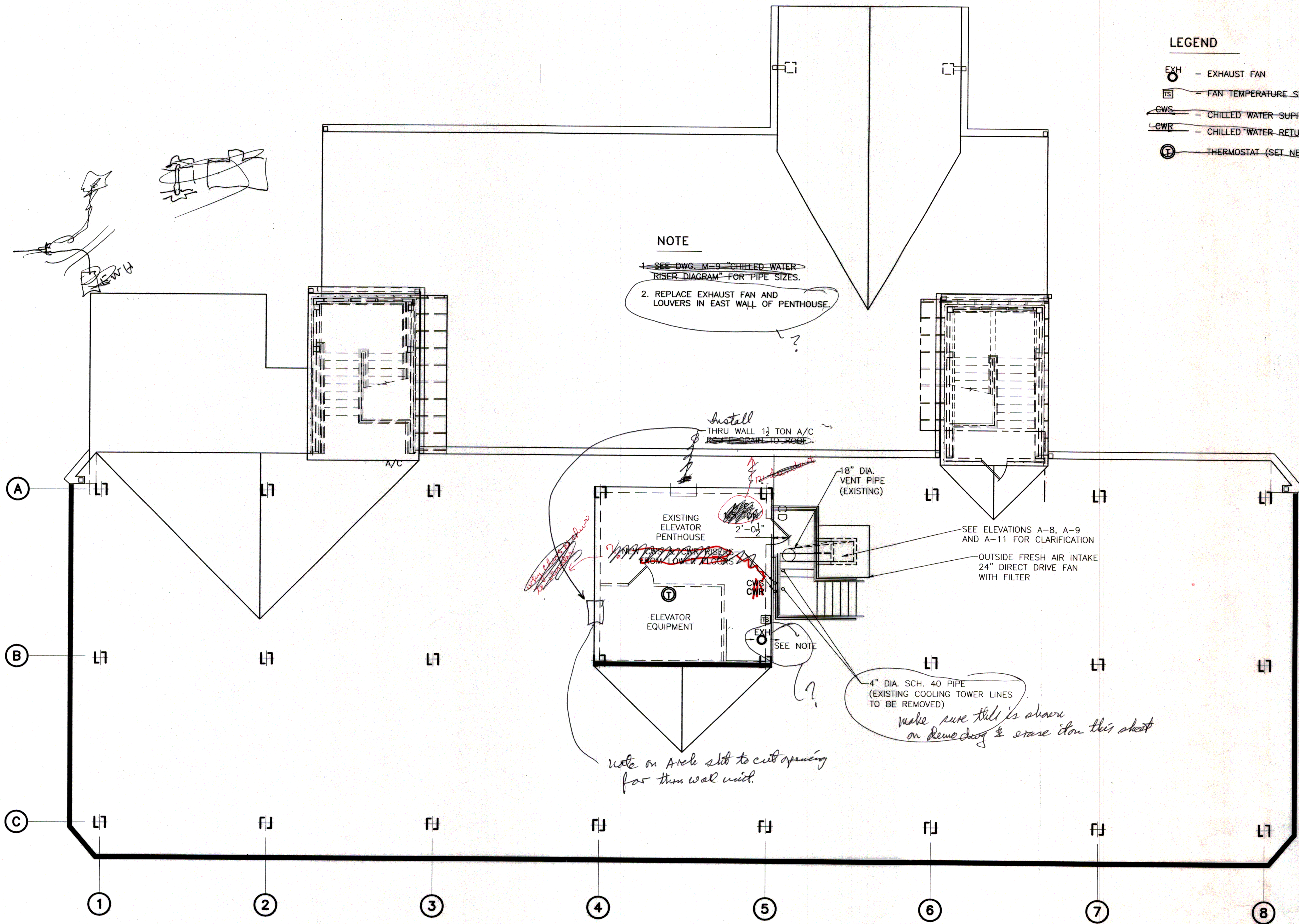
ROOF MECHANICAL PLAN SCALE: 3/16" = 1'-0"
