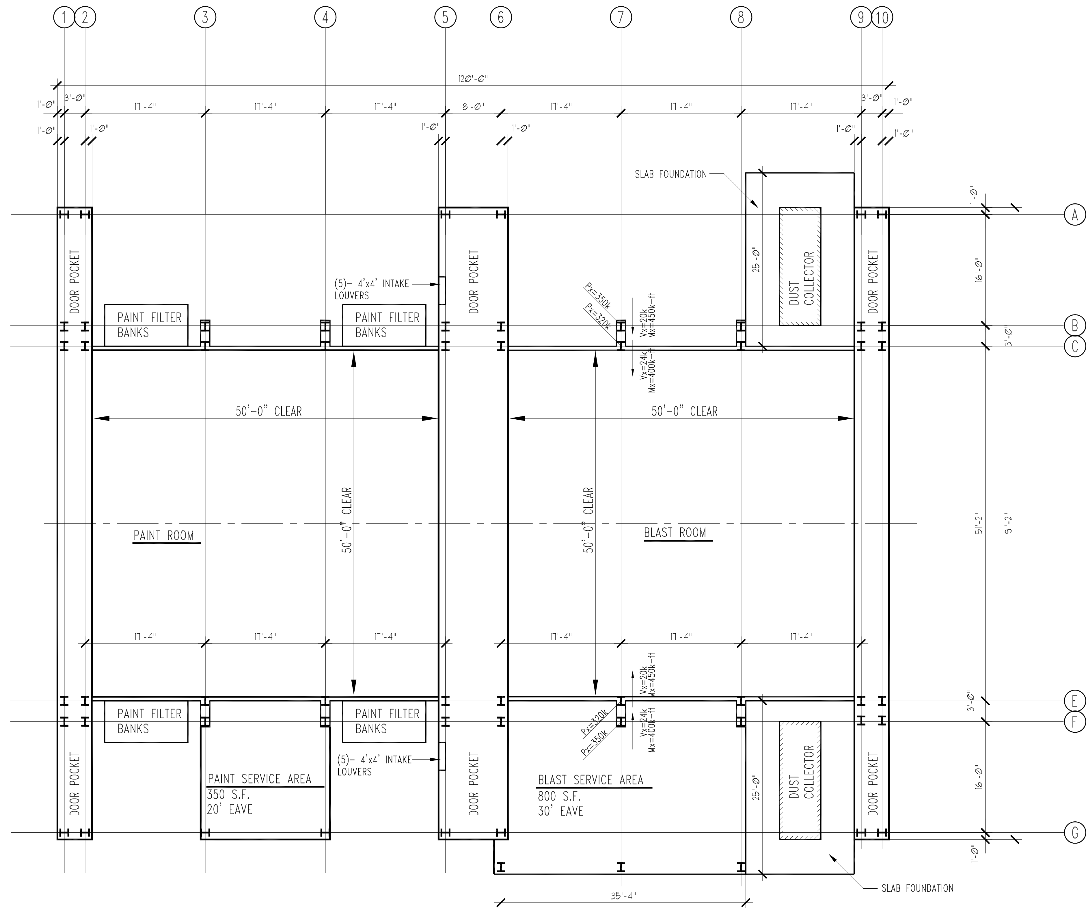
A SCHEMATIC LAYOUT S1.00
