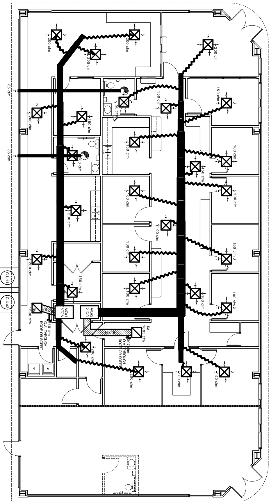
MECHANICAL PLAN SCALE 3/16" = 1'
