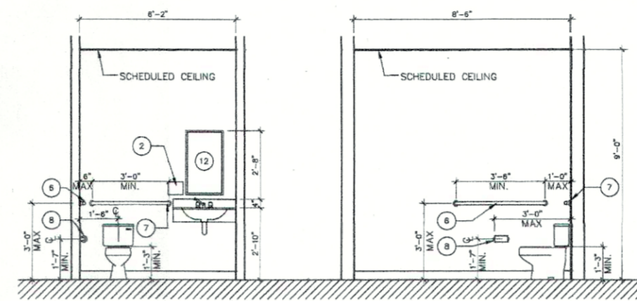
3A 3B INTERIOR ELEVATIONS 3 STAFF HC TOILET ROOM 148 SCALE: 3/8"=1'-0" A-4.02
