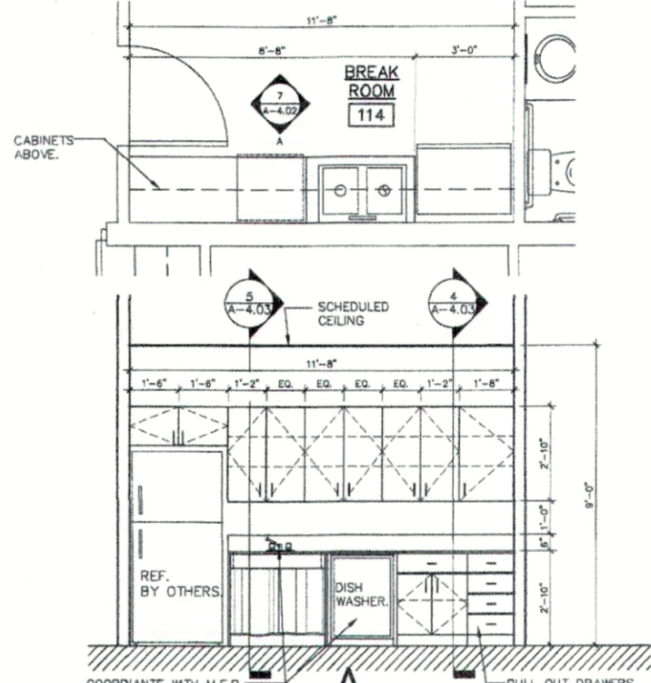
BREAK ROOM 114 7 ENL. PLAN AND INT. ELEV. SCALE: 3/8"=1'-0" A-4.02
