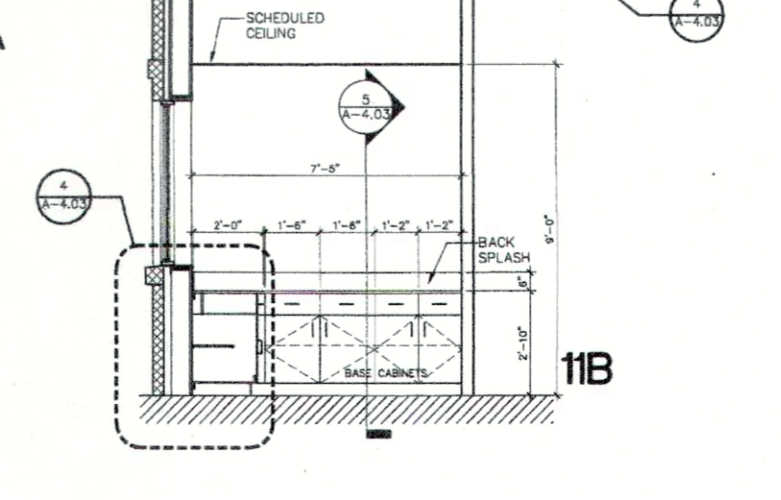
LAUNDRY STORAGE 115 11 ENLARGED PLAN AND INT. ELEV.S SCALE: 3/8"=1'-0" A-4.02
