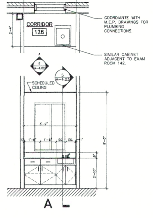
CORRIDOR 128 8 ENLARGED PLAN AND INT. ELEV. SCALE: 3/8"=1'-0" A-4.02
