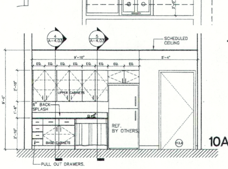
PANTRY / BREAK ROOM 113 10 ENLARGED PLAN AND INT. ELEV.S SCALE: 3/8"=1'-0" A-4.02
