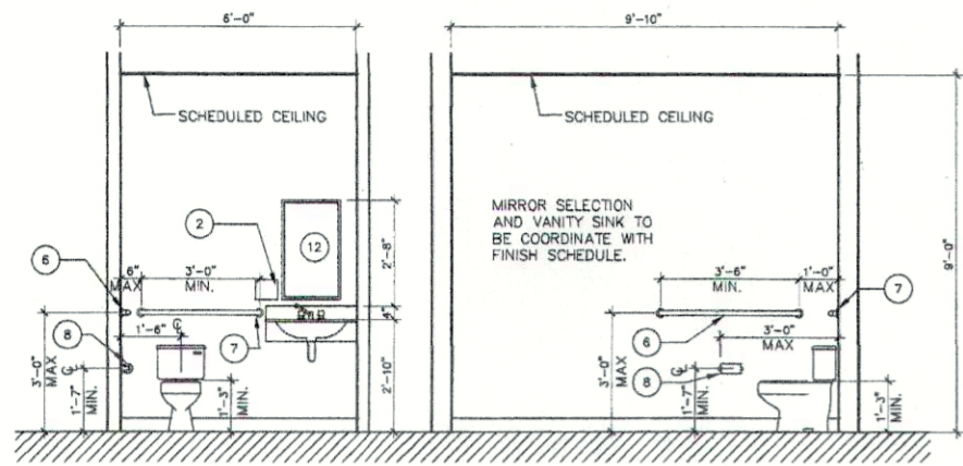
1A 1B INTERIOR ELEVATIONS 1 HC TOILET ROOM 108 SCALE: 3/8"=1'-0" A-4.02
