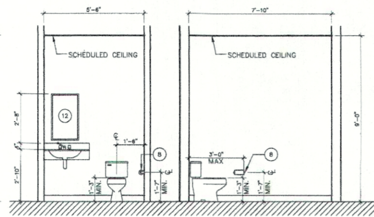
2A 2B INTERIOR ELEVATIONS 2 STAFF TOILET ROOM 104 SCALE: 3/8"=1'-0" A-4.02
