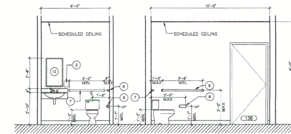
4A 4B INTERIOR ELEVATIONS 4 FEMALE HC TOILET ROOM 136 SCALE: 3/8"=1'-0" A-4.02
