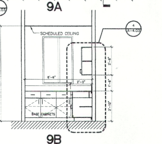
NURSES' STATION 106 9 ENLARGED PLAN AND INT. ELEV.S SCALE: 3/8"=1'-0" A-4.02
