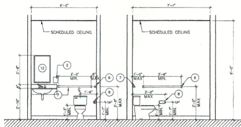
5A 5B INTERIOR ELEVATIONS 5 MALE HC TOILET ROOM 135 SCALE: 3/8"=1'-0" A-4.02
