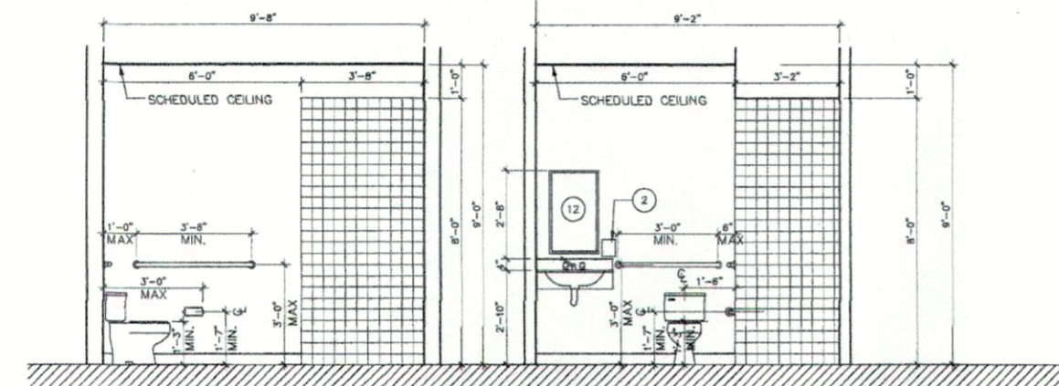
6A 6B INTERIOR ELEVATIONS 6 DOCTOR'S SHOWER ROOM 126 SCALE: 3/8"=1'-0" A-4.02
