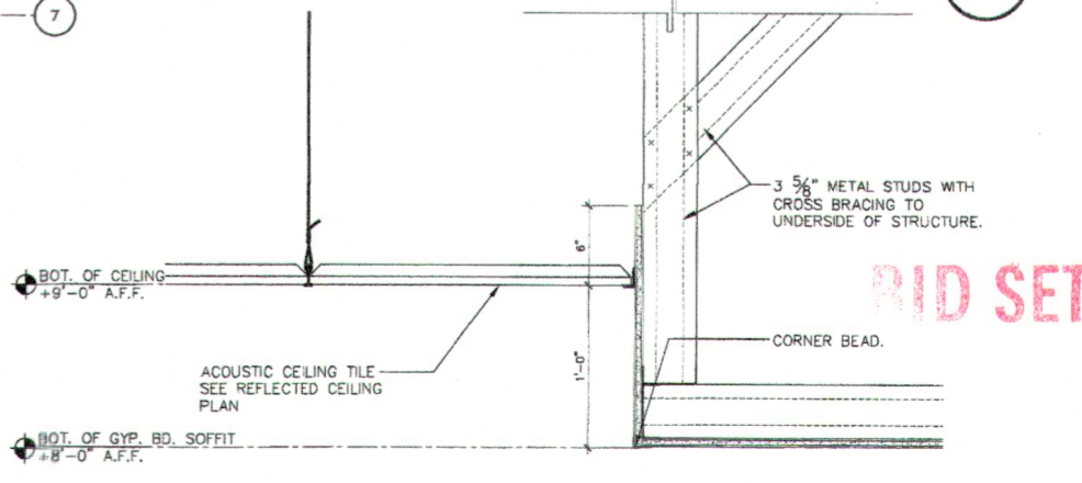
BULKHEAD DETAIL 2 SCALE: 1-1/2" = 1'-0"
