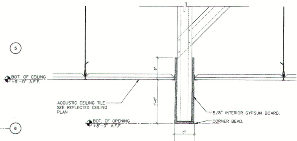
BULKHEAD DETAIL 2 SCALE: 1-1/2" = 1'-0"
