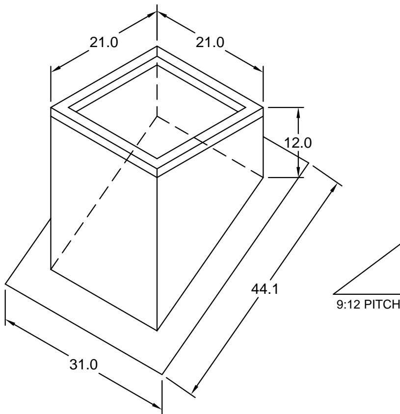
ISOMETRIC VIEW
