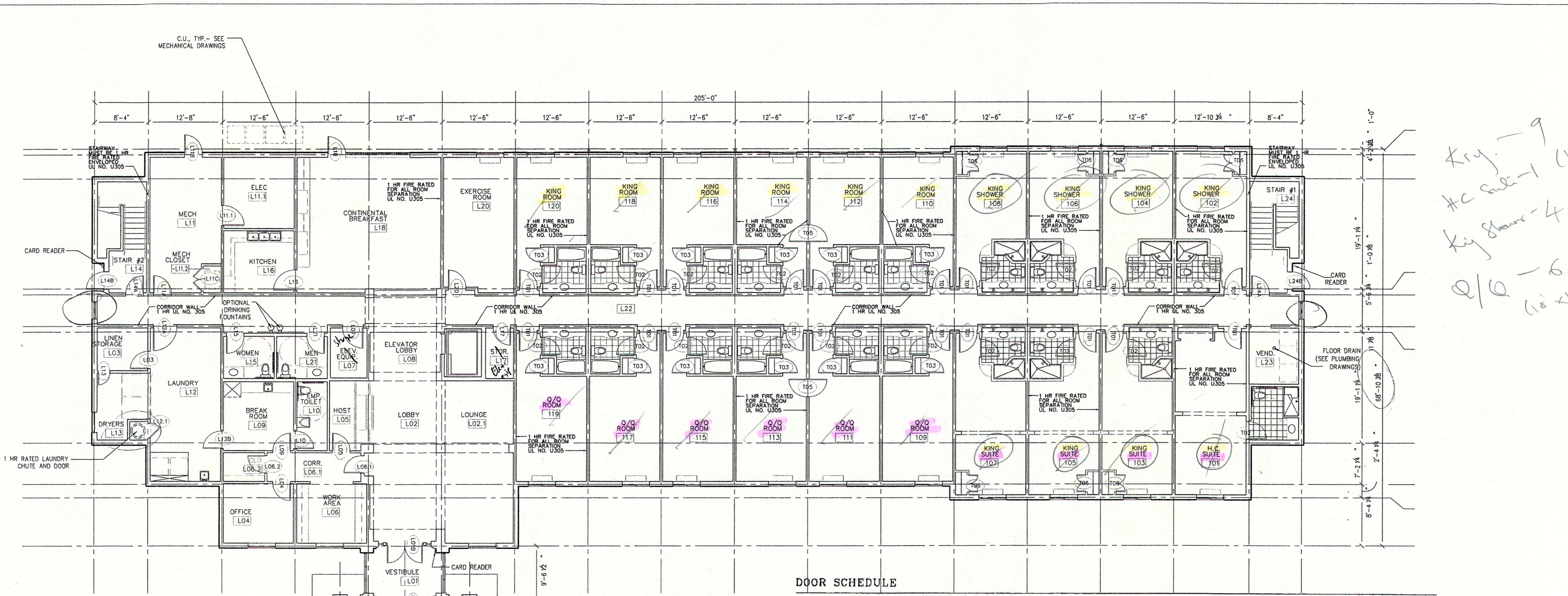
LOBBY LEVEL PLAN SCALE: 3/32" = 1'-0"
