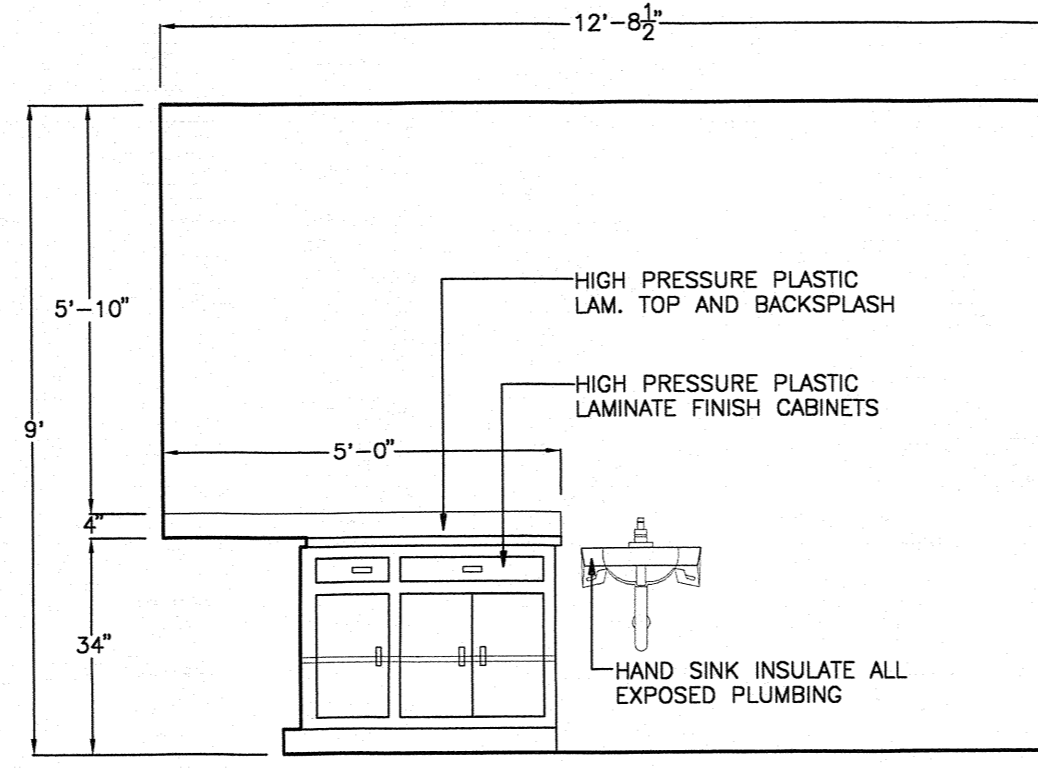
6 FOOD PREP ELEVATION SCALE: 3/8" = 1'-0"
