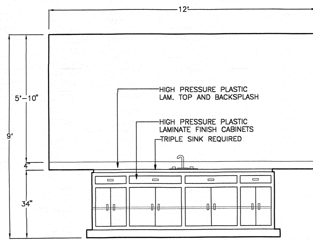
5 FOOD PREP ELEVATION SCALE: 3/8" = 1'-0"
