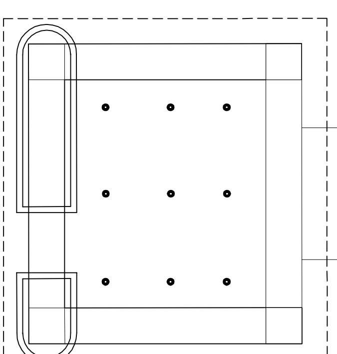
GROUND FLR REFLECTED CEILING PLAN SCALE: 1/8"=1'-0"
