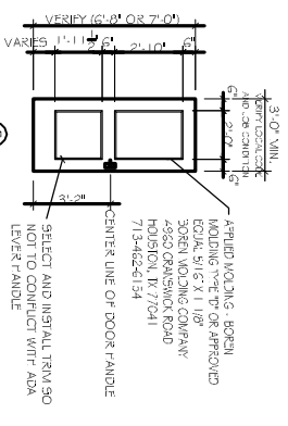
HOLLOW CORE 2 PANEL COLONIST
