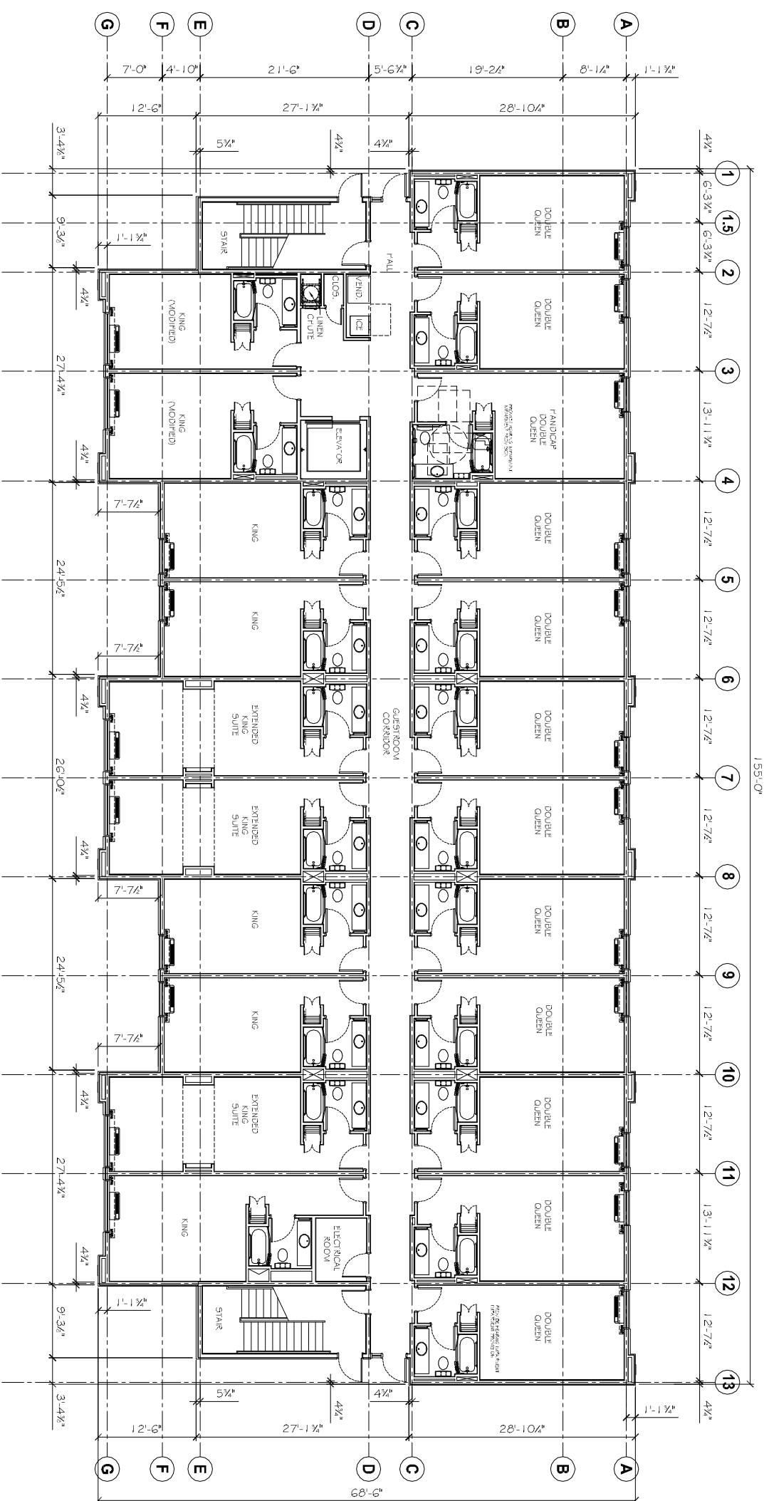
SECOND & THIRD FLOOR PLAN-SCHEME FOUR SCALE: 1/8" = 1'-0" 22 GUEST ROOMS
