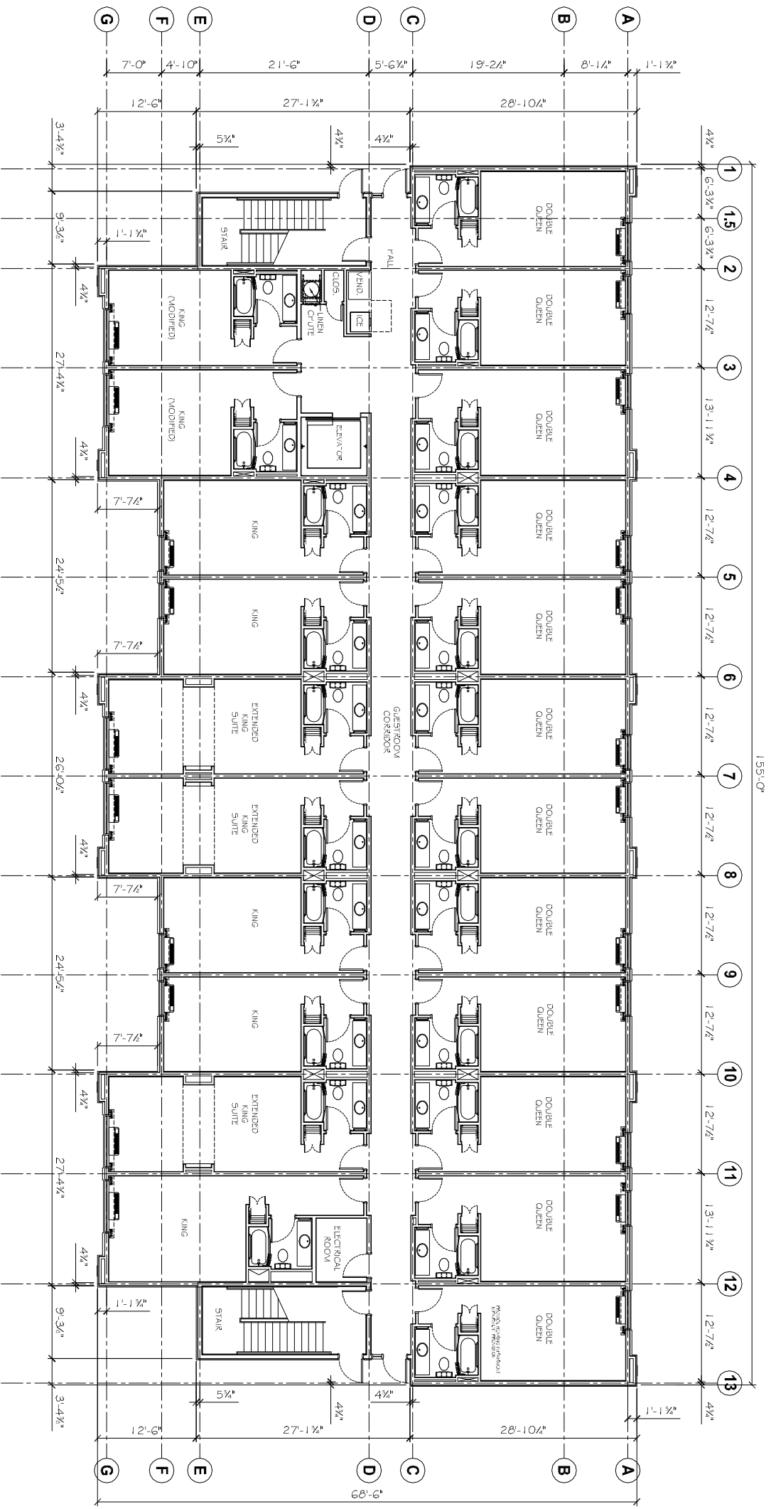
FOURTH FLOOR PLAN-SCHEME FOUR SCALE: 1/8"=1'-0" 22 GUESTROOMS
