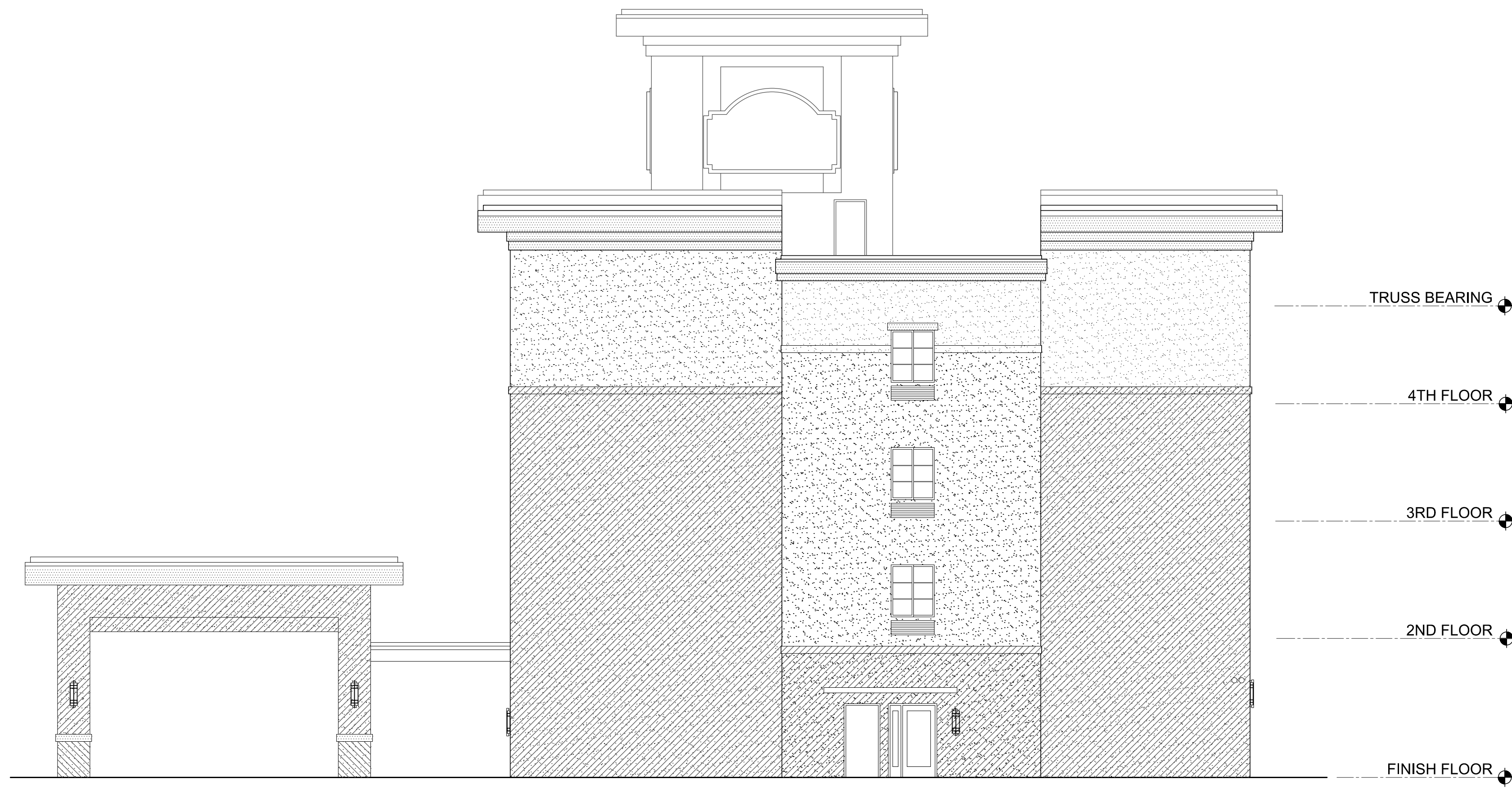
Ø2-SIDE ELEVATION
