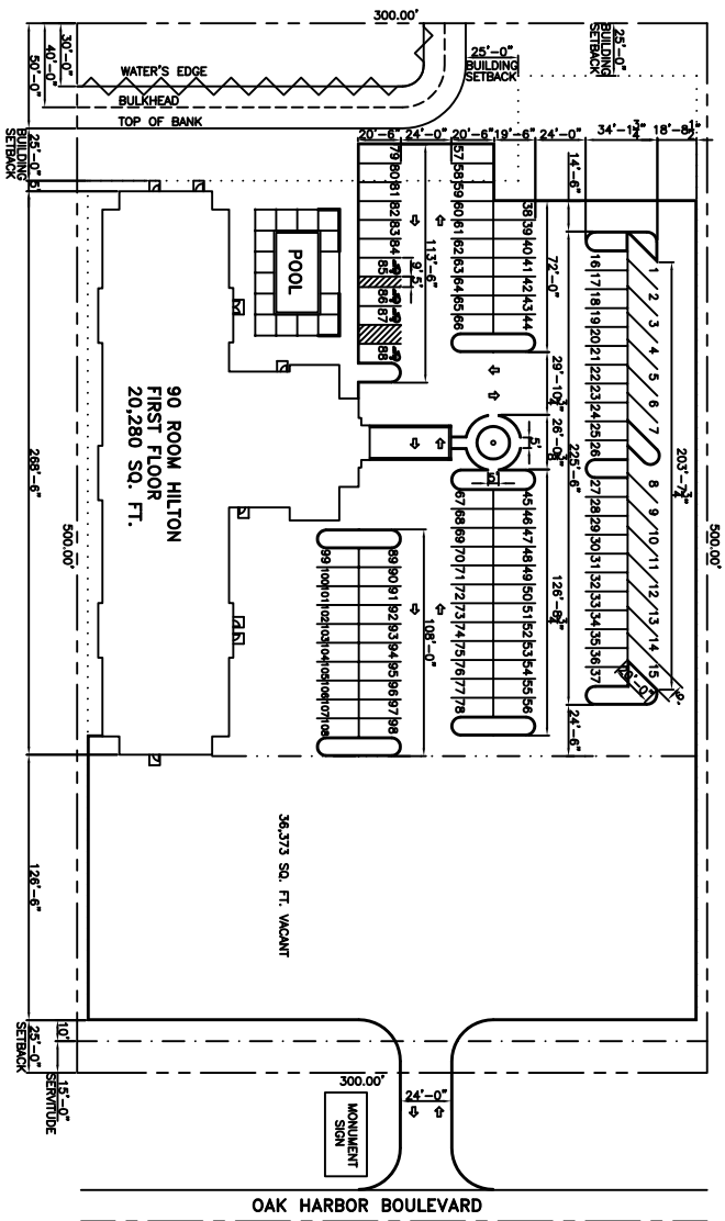
SITE PLAN SCALE: 1"=30'-0"
