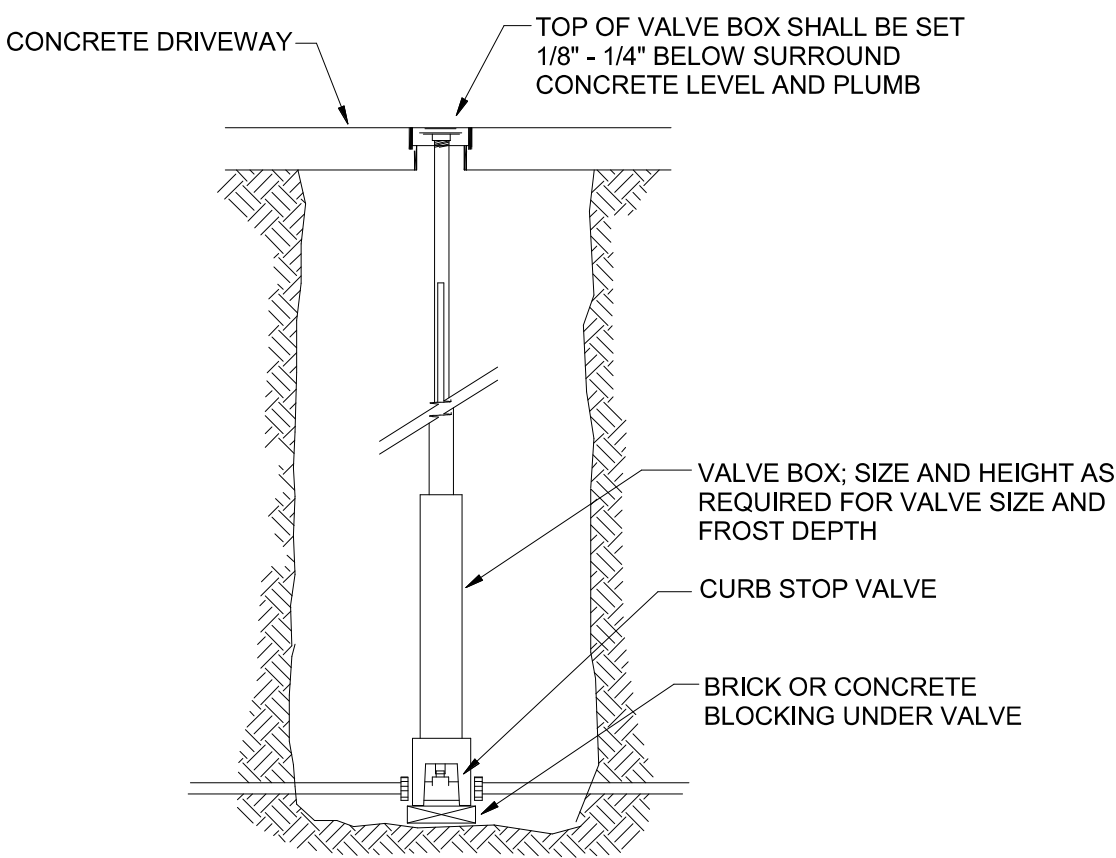
2 CURB BOX DETAIL NTS
