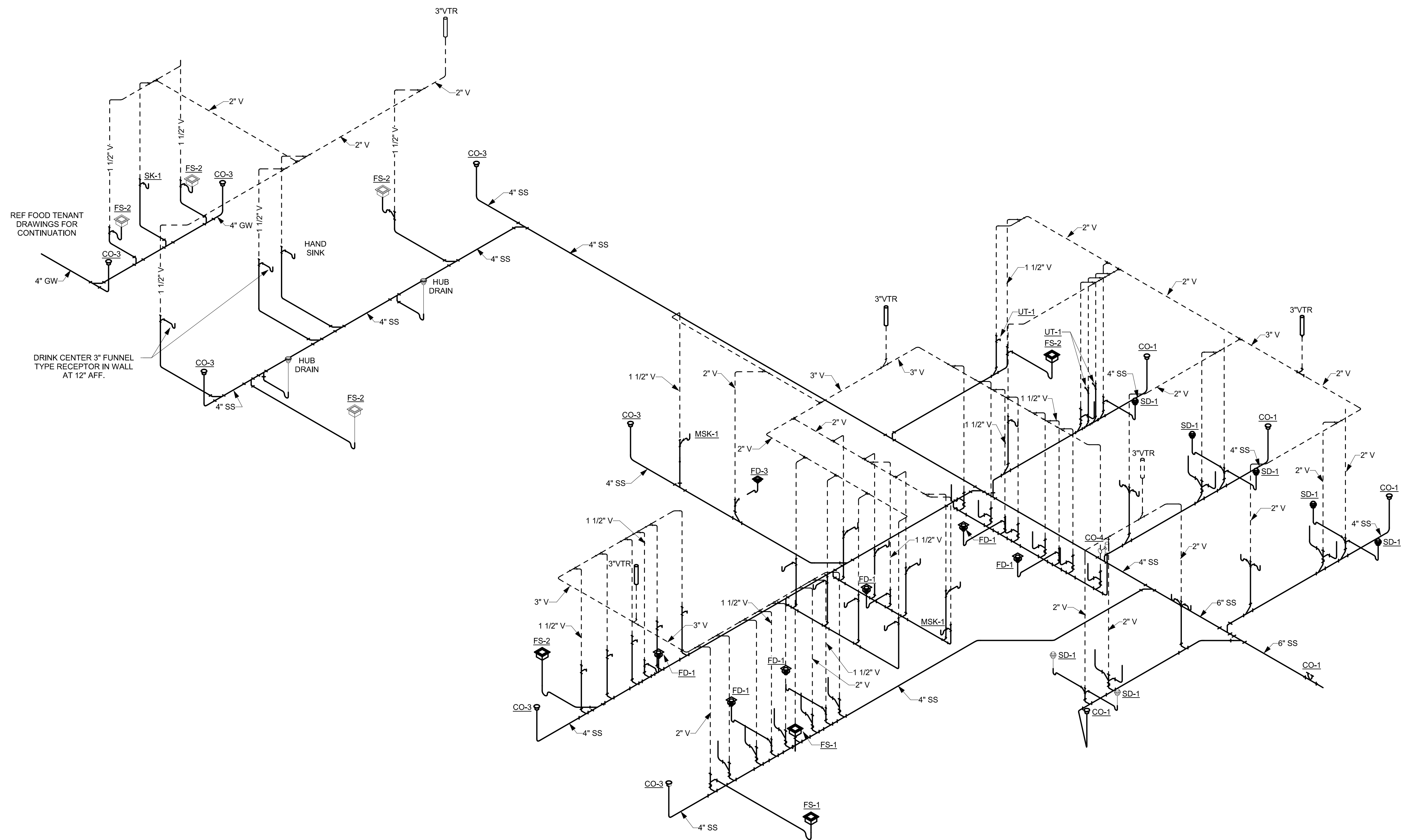
1 WASTE AND VENT RISER NTS
