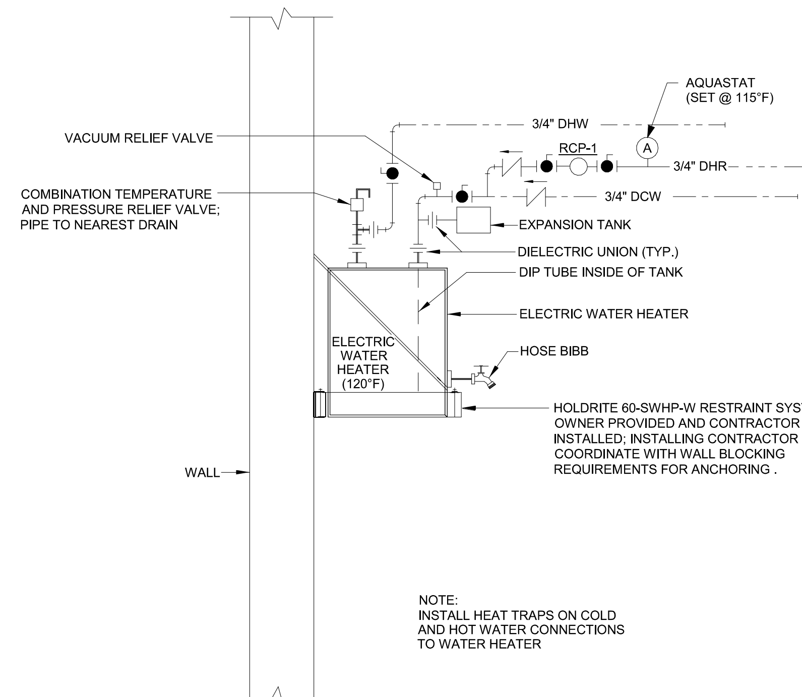
1 WALL MOUNTED ELECTRIC WATER HEATER NTS
