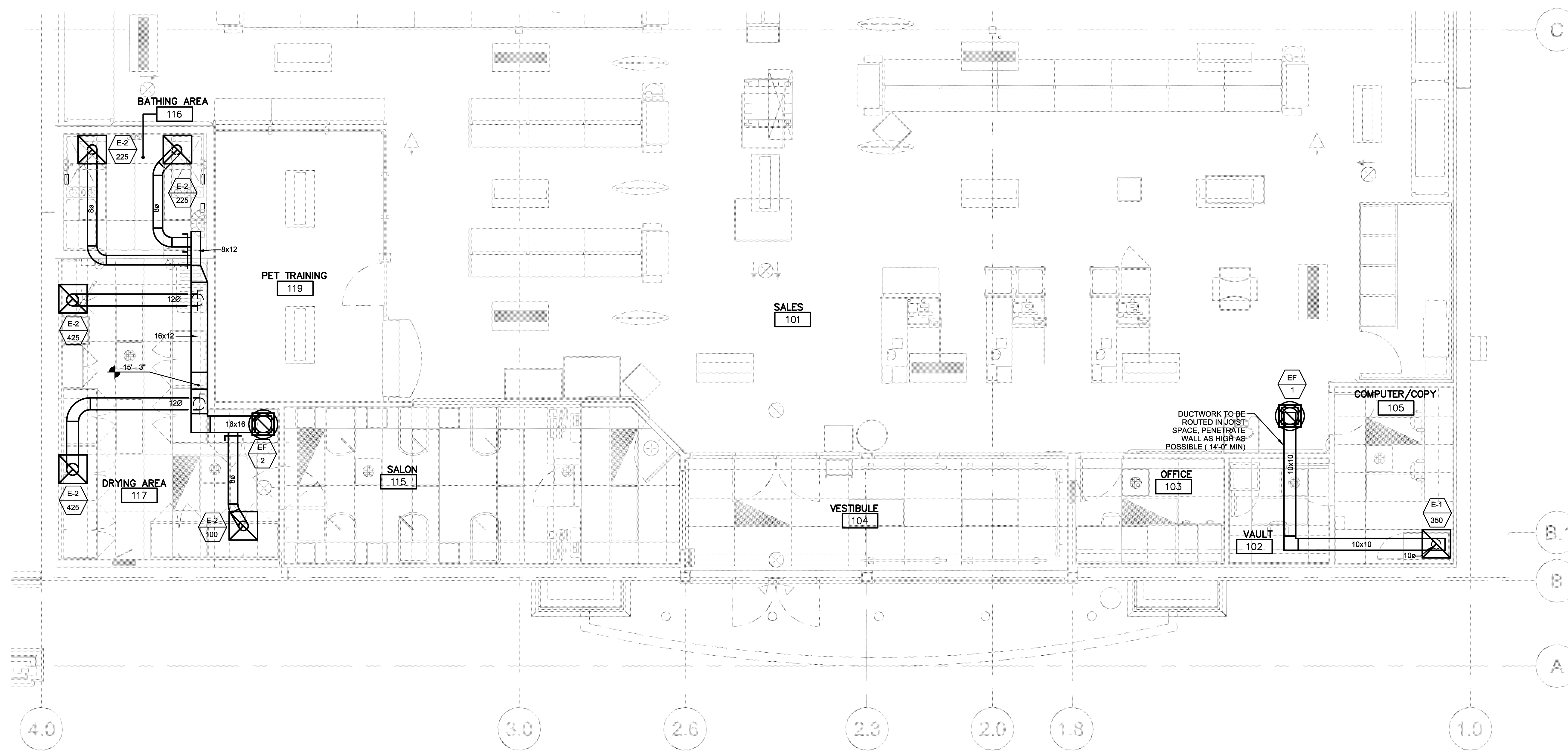
2 ENLARGED MECHANICAL SALON / OFFICE EXHAUST PLAN M1.1 SCALE: 1/4" = 1'-0" NORTH
