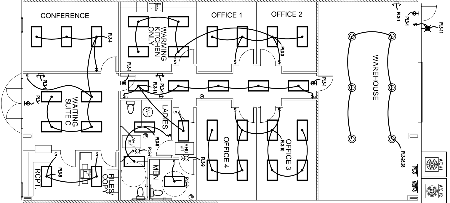
LIGHTING PLAN SUITE C SCALE: 3/16"=1'-0"
