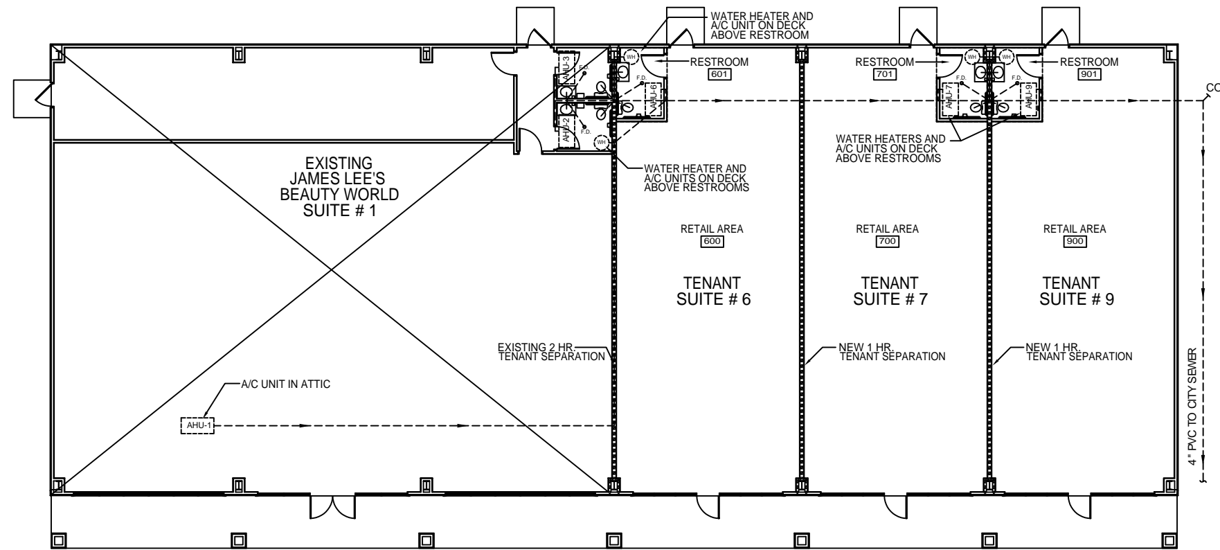
PLUMBING PLAN SCALE: 1/8"=1'
