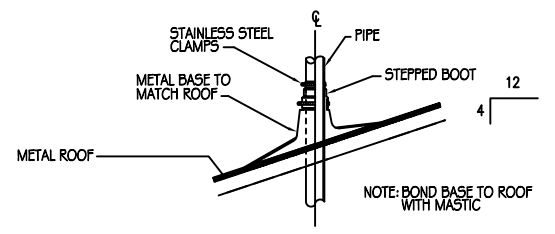
VENT THRU ROOF DETAIL N.T.S.
