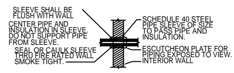
TYPICAL INTERIOR WALL SLEEVE DETAIL N.T.S.
