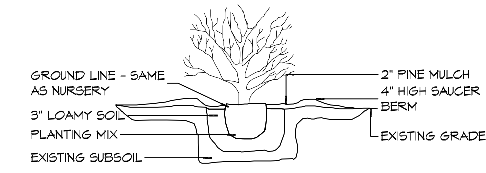
B TYPICAL SHRUB PLANTING
