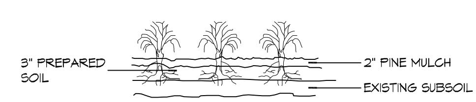
A GROUND COVER
