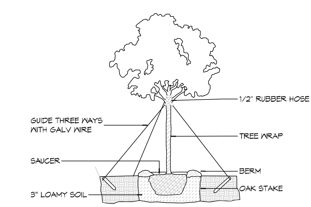
C TYPICAL TREE PLANTING NOTE: ALWAYS PLANT EQUAL TO OR 1" - 2" ABOVE GROUND.
