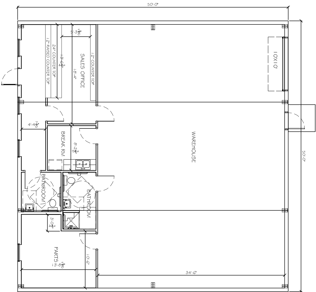
FLOOR PLAN SCALE: 1/4" = 1'
