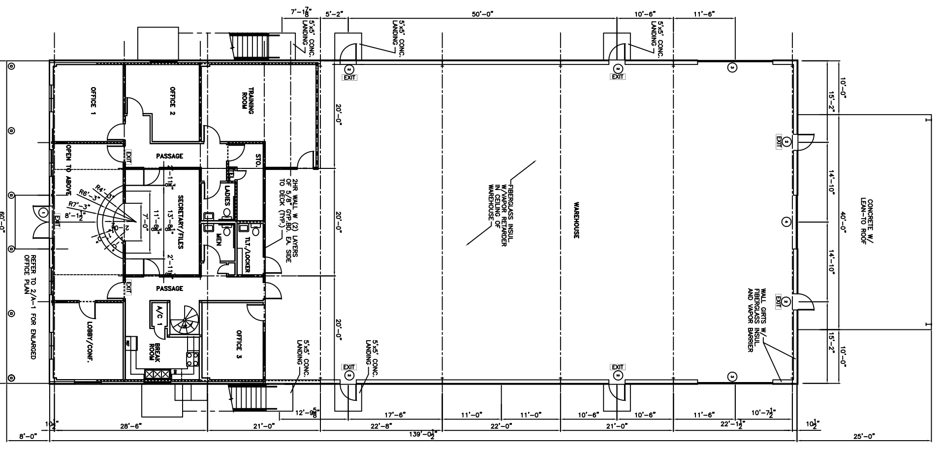
1 OVERALL FIRST FLOOR PLAN 1/8"=1'-0"
