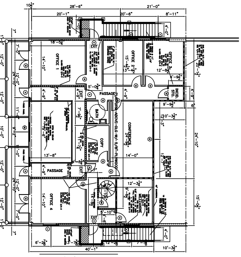
2 ENLARGED OFFICE PLAN SECOND FLOOR 1/8"=1'-0"
