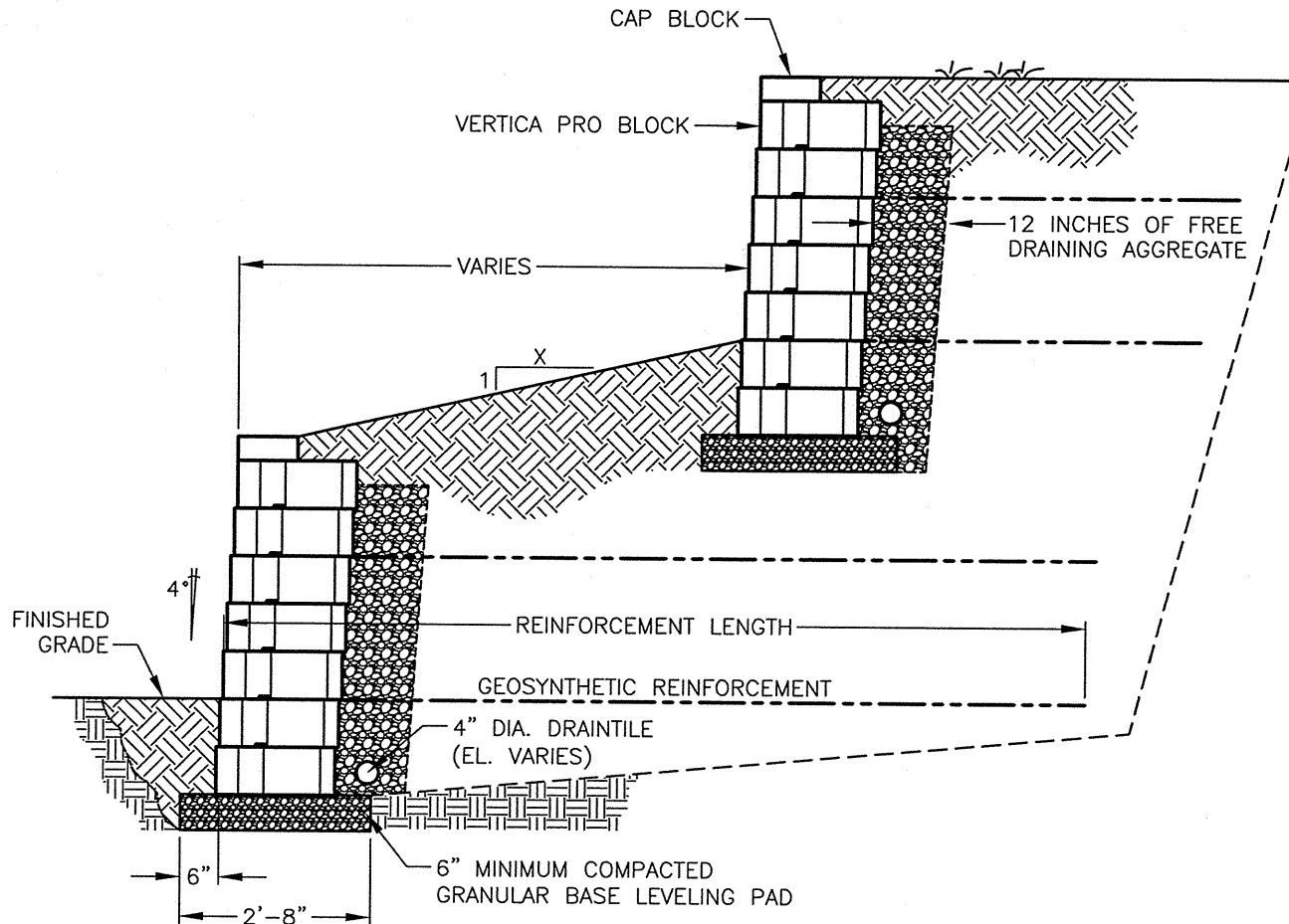
X WX ANCHOR VERTICA PRO ® TERRACED WALL DETAILS (SCALE: 3/8" = 1'-0")
