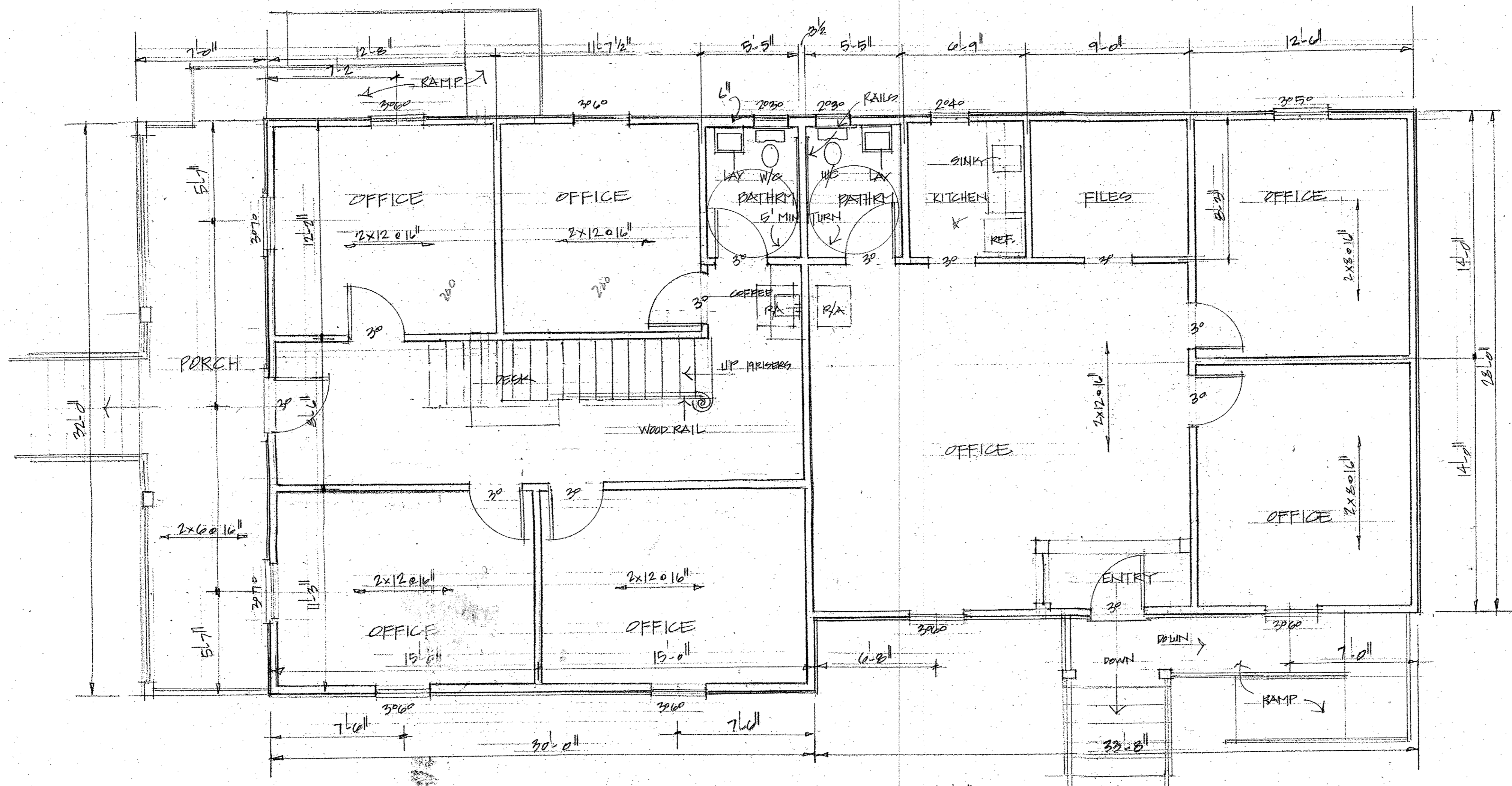
FLOOR PLAN 1/4" = 1'-0"
